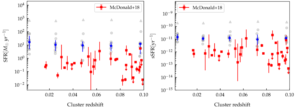
Fig. 1. BCG SFR (left panel) and specific SFR (right panel) in simulations (grey points) and in the observations from McDonald et al. 2018 (red points). Measures are done within 30 pkpc in 2D. The slight offset of the grey point is for visualization only. Median, 16 th , and 84 th percentiles are shown in blue.
