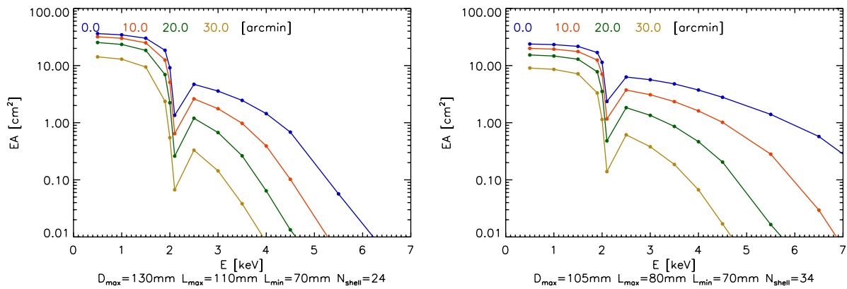
Fig. 8. EA as a function of energy for various off-axis locations (on-axis: blue; 10': orange; 20': green; 30': yellow) for the large ( left ) and small ( right ) designs. This is a different projection of the information presented in Fig. 7.
