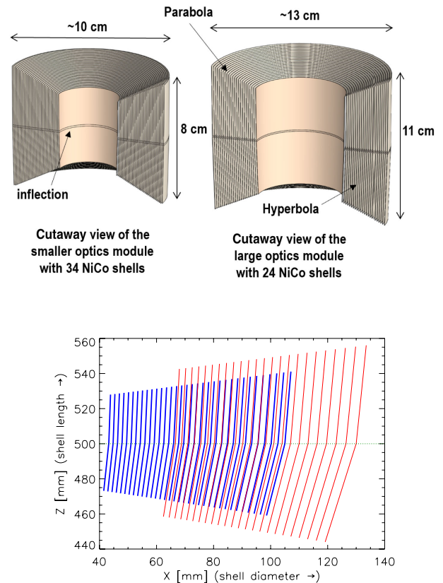
Fig. 4. Sketches of the CubeX tapered configurations drawn to scale. The cutaway views of the small (top left) and large (top right) configurations are also shown. The lower panel shows a line drawing cutouts of the profiles, with the large (red) and compact (blue) shells superposed. The horizontal dotted line indicates the focal length.
