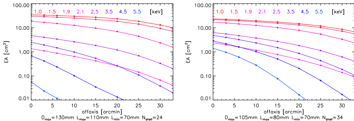
Fig. 7. Effective area (EA) as a function of off-axis location for the large ( left ) and small ( right ) designs. The different colored curves are for different photon energies as in Fig. 5. A different projection of the same information, EA versus energy for different off-axis angles is shown in Fig. 8.
