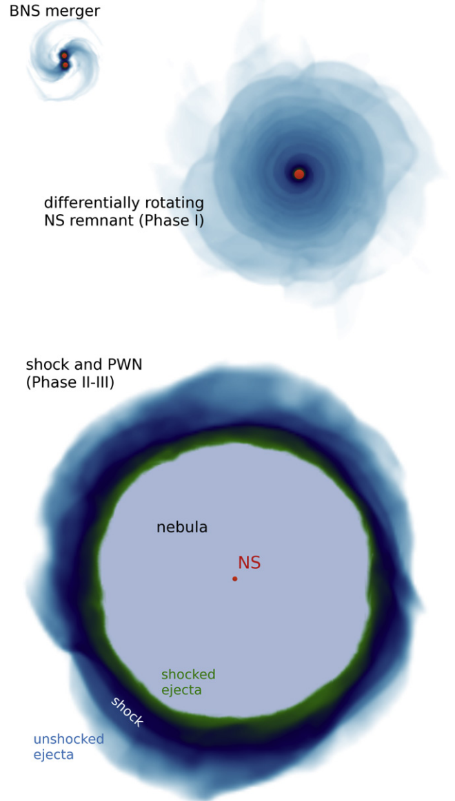
Figure 1. Evolution of the system according to the proposed scenario (with increasing spatial scale). A BNS merger (top left) forms a differentially rotating NS that emits a baryon-loaded wind (Phase I). The NS eventually settles down to uniform rotation and inflates a pulsar wind nebula (or simply “nebula”) that sweeps up all the ejecta material into a thin shell (Phase II). Spin-down emission from the NS continues while the nebula and the ejecta shell keep expanding (Phase III).
