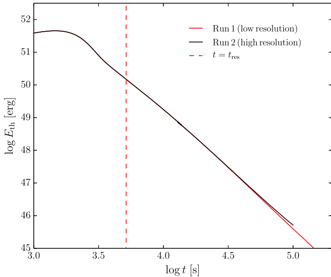
Figure 3. Evolution of the internal energy E_{\text{th}} of the ejecta shell in Phase III according to a run using the evolution scheme described in this section (Run 1) and a run using additional mesh refinement to evolve Equation (14) up to late times (Run 2). The dashed red line indicates the time of transition t = t_{\text{res}} to the modified evolution scheme for Run 1.
