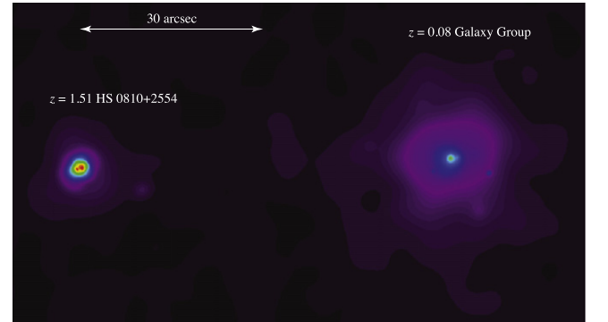
Figure 12. Adaptively smoothed image of the 100 ks Chandra observation of HS 0810+2554. Our spectral analysis confirms our previous result, which was based on a 5 ks exposure (Chartas et al. 2014), that the extended emission 58'' west of HS 0810+2554 is produced by a galaxy group at z \sim 0.08 .
