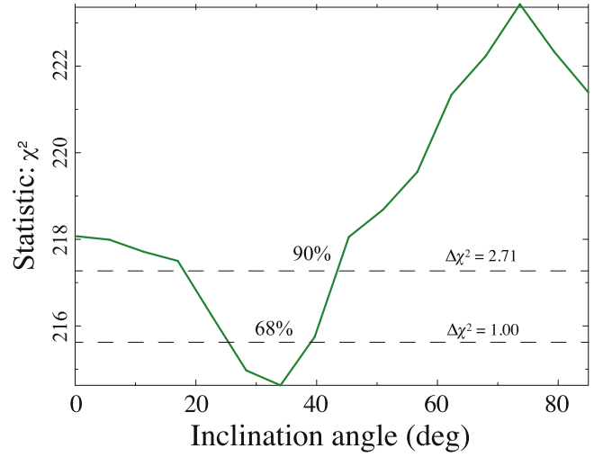
Figure 11. Fits to the XMM-Newton spectrum of HS 0810+2554 constrain the inclination angle of the accretion disk (model 7 of Table 5). The \chi^2 confidence plot indicates an inclination angle of <45^{\circ} (90% confidence), which is consistent with models that posit NALQSOs as objects observed at relative low inclination angles.
