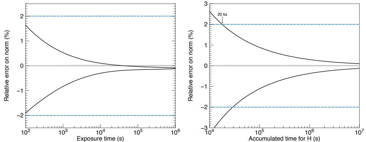
Figure 4. ( Left ) Relative error (%) on the value of the NXB normalisation as a function of time (s) when using the CryoAC technique with an estimate of H measured over 100 ks obtained for 1 000 iterations. The bias on the correction is due to the finite accumulated time to estimate of H . ( Right ) Relative error made on the CryoAC correction as a function of accumulated time (in s) used to estimate the transfer function matrix H . Dashed lines represent the 2% threshold.
