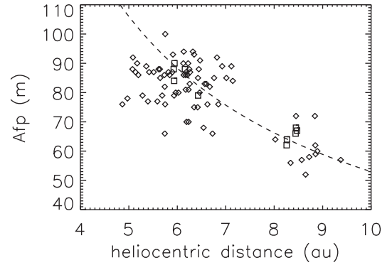
Figure 3. Afp of comet C/2017K2 versus the heliocentric distance r_h measured within a sky-projected coma radius \rho_0 = 5 \times 10^4 \text{ km} . Diamonds: observations of the CARA network. Squares: observations at Loiano Observatory. Dashed line: best fit of Loiano’s data constrained by the dust tail model (Table 5).
