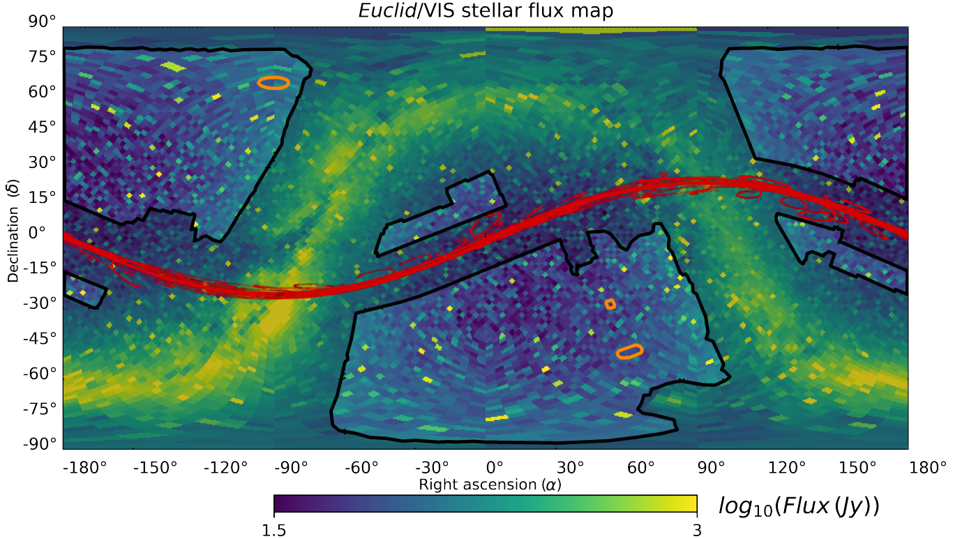
Fig. 1. Euclid /VIS stellar flux density map, based on Gaia (Gaia Collaboration 2016, 2018) and Sahlmann et al. (2016) catalogs: Black contours: footprint of a proxy of the Euclid /VIS Survey (Scaramella et al. 2021). The darkened regions, corresponding to the peak of the Milky Way emission, lie outside the footprint. The three regions marked with orange contours correspond to the Deep North, Deep South, and Deep Fornax fields. Color background: stellar flux density per HEALpix cell. The brightest region corresponds to the Galactic plane, a region avoided by the Euclid footprint. See the bottom color bar for the scaling. Red lines: projected trajectories of the main Solar System bodies (Mercury, Venus, Earth, Mars, Jupiter, Saturn, Uranus, and Neptune) as seen by Euclid during the mission, following the ecliptic plane (Giorgini et al. 2001).
