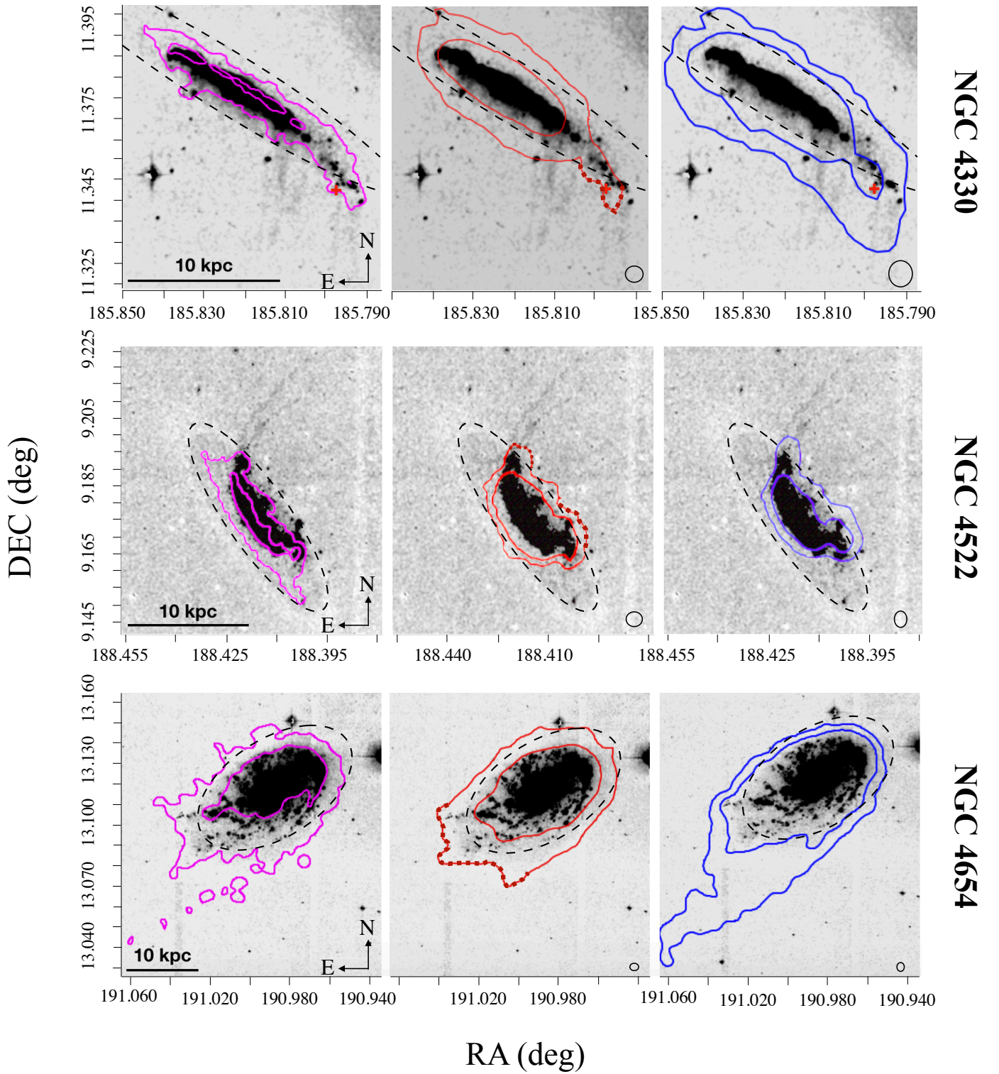
Fig. 2. Smoothed H\alpha VESTIGE images of NGC 4330 ( top ), NGC 4522 ( centre ), and NGC 4654 ( bottom ) compared with the GALEX FUV emission (magenta contours), SPIRE 250 \mu\text{m} emission (red contours), and VIVA HI emission (blue contours). The faintest emissions from the SPIRE 250 \mu\text{m} data are at surface brightness levels of 0.6 \text{ MJy sr}^{-1} , while the HI contour levels reach column densities values of \Sigma_{\text{HI}} = 2 \times 10^{19} \text{ cm}^{-2} . Dotted black ellipses trace the extensions of the galaxies' optical discs. The regions of the tails outside the optical disc are considered for our photometric analysis (red dotted contours). Linear scales and synthesised beam sizes are shown in the bottom-left and bottom-right corners, respectively.
