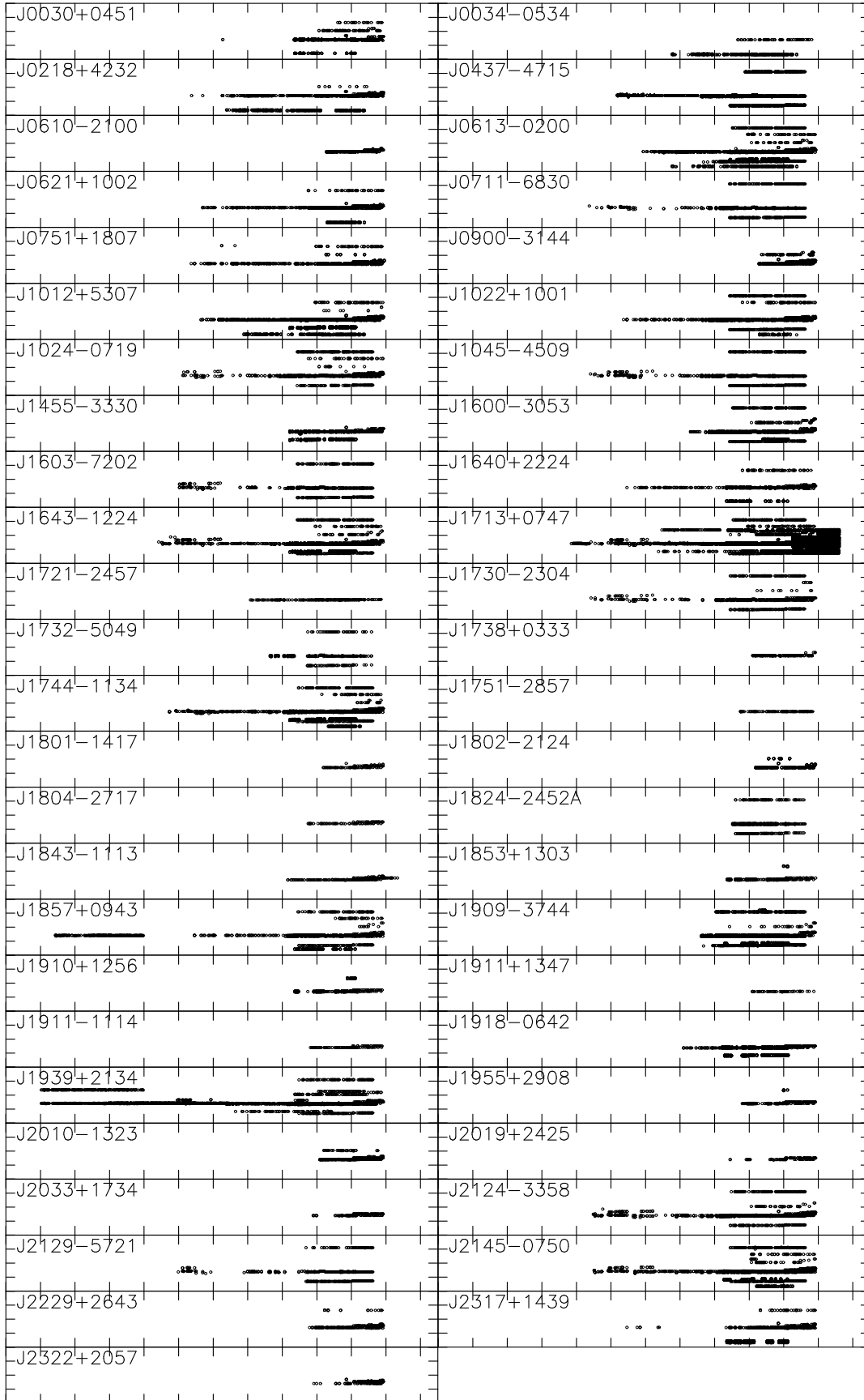
Figure 4. Plot of temporal and frequency coverage for all pulsars. The ranges of each sub-plot are identical and cover the MJD-range 45000 to 57500 (31 January 1982 to 22 April 2016) in X and 0 to 4 GHz in Y. Tick marks are at 1000-day and 1-GHz intervals. Note that only the centre frequency of each ToA is plotted (i.e. the bandwidth is ignored) and that many pulsars have only a few years of data at a single frequency. © 2015 RAS, MNRAS 000 , 1–25
