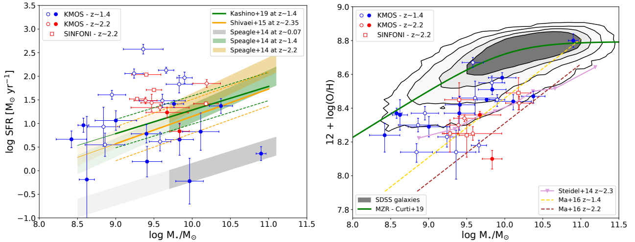
Figure 6. Left Panel: Distribution of our galaxy sample in the SFR vs M_* plane. Symbols and colours are the same as in Fig. 5. Both SFR and M_* measurements are corrected for lensing magnification and the error bars account for the uncertainties associated to the reddening correction and the statistical uncertainty on the magnification itself. The representative star-forming main sequence (SFMS) at redshift 0.07, 1.4 and 2.2 from Speagle et al. (2014) is represented by grey, green and yellow shaded regions respectively, with a nominal intrinsic scatter of 0.2 dex. The best-fit to SFMS (based on dust corrected \text{H}\alpha -based SFR) from Kashino et al. (2019) (FMOS Survey, z \sim 1.4 ) and Shivaiei et al. (2015) (MOSDEF Survey, z \sim 2.3 ) are also plotted with green and golden solid lines, with an observational scatter of 0.3 and 0.36 dex respectively. All SFRs are reported to a common Chabrier (2003) IMF. Right Panel: Relationship between stellar mass and gas-phase metallicity for our sample, derived with the C17 and C19 calibrations as described in the text. Colors and symbols are the same as in the left panel. The region within grey contours encloses the 68%, 84% 95% and 99% of the distribution of local SDSS galaxies in the M_* vs O/H plane, with abundances calculated from the same C17 and C19 calibrations, and the relative best-fit MZR to median points in bins of stellar mass from Curti et al. (2019) is shown in green. We also plot the MZR at z \sim 2.3 from Steidel et al. (2014) in bins of stellar mass, shown in violet, as obtained from the O3N2 diagnostic rescaled to the C17 calibrations. All these metallicity measurements are consistent with the abundance scale defined by the T_e method. For comparison, we also show, with yellow and brown dashed curves respectively, the predicted MZR at z = 1.4 and z = 2.2 from high-resolution FIRE simulations, as presented in Ma et al. (2016). In agreement with the prescriptions of an evolving MZR, our galaxies are characterised by lower metallicities, at fixed M_* , compared to local galaxies (0.24 and 0.36 dex lower on average than the local MZR for z \sim 1.4 and z \sim 2.2 sources respectively). However, C17-C19 calibrations provide higher metallicities compared to the abundance scale defined by both Ma et al. (2016) simulations at the reference redshift, possibly due to the uncertainties affecting the stellar yields adopted in the simulations.
