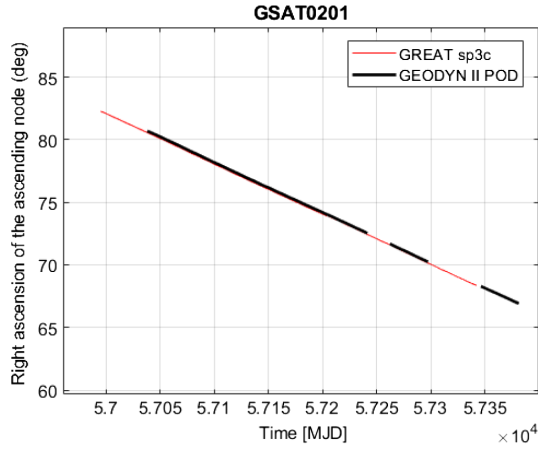
F43:1 FIG. 43. Comparison between GEODYN II POD (black) and F43:2 GREAT sp3c precise orbit (red): long-term evolution of the F43:3 RAAN of GSAT0201.
