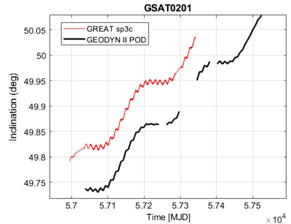
F42:1 FIG. 42. Comparison between GEODYN II POD (black) and F42:2 GREAT sp3c precise orbit (red): long-term evolution of the F42:3 inclination of GSAT0201.
