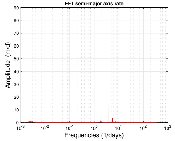
F26:1 FIG. 26. GSAT0202 (E14): spectral analysis for the rate of the F26:2 semimajor axis long-period effects of direct SRP.
