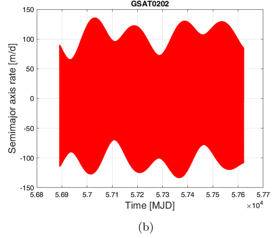
F19:1 FIG. 19. Long-term evolution of the semimajor axis rate of the satellites. (a) GSAT0201: long-term evolution of semi-major axis F19:2 rate \dot{a} . (b) GSAT0202: long-term evolution of semi-major axis rate \dot{a} .
