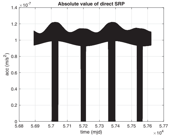
FIG. 9. GSAT0201 (E18): absolute value of the acceleration due to direct SRP.
