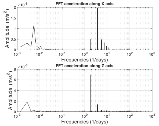
FIG. 18. GSAT0201 (E18): spectral analysis of the SRP accelerations along the X (top) and Z (bottom) directions also showing the long-period effects of direct SRP.
