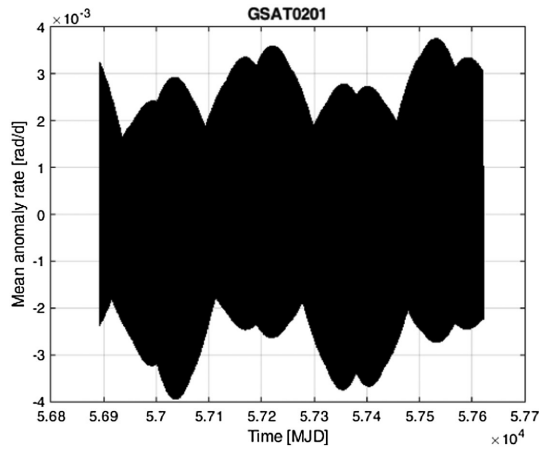
F24:1 FIG. 24. GSAT0201: long-term evolution of the Mean anomaly rate in \eta: \dot{\eta} . F24:2
