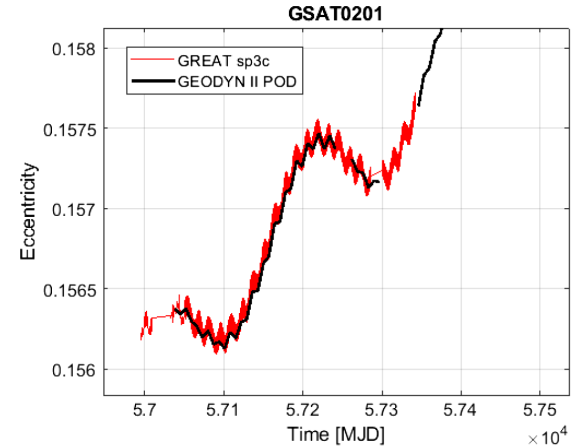
F41:1 FIG. 41. Comparison between GEODYN II POD (black) and F41:2 GREAT sp3c precise orbit (red): long-term evolution of the F41:3 eccentricity of GSAT0201.
