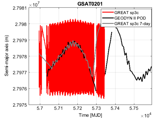
F40:1 FIG. 40. Comparison between GEODYN II POD (black) and F40:2 GREAT sp3c precise orbit (red): long-term evolution of the F40:3 semimajor axis of GSAT0201.
