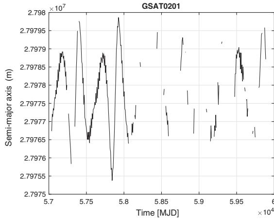
F35:1 FIG. 35. GEODYN II POD of GSAT0201: long-term evolution F35:2 of the semimajor-axis.
