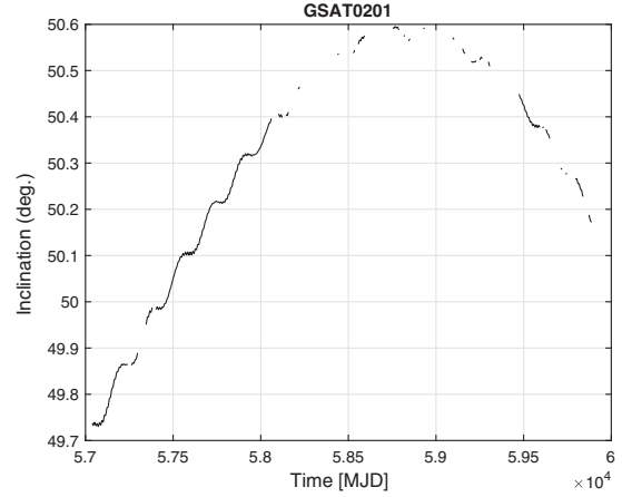
F37:1 FIG. 37. GEODYN II POD of GSAT0201: long-term evolution F37:2 of the inclination.
