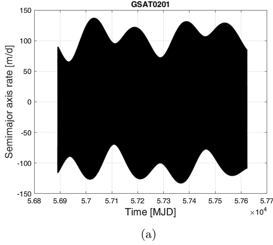
F19:1 FIG. 19. Long-term evolution of the semimajor axis rate of the satellites. (a) GSAT0201: long-term evolution of semi-major axis F19:2 rate \dot{a} . (b) GSAT0202: long-term evolution of semi-major axis rate \dot{a} .
