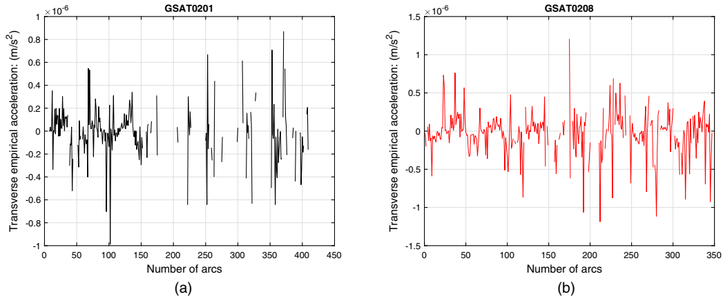
F34:1 FIG. 34. Empirical transverse (sine component) acceleration (m/s 2 ), estimated for each arc of the POD. Outliers more than three F34:2 standard deviations from the mean of the acceleration values have been removed. (a) GSAT0201: empirical transverse acceleration per F34:3 arc: T_s amplitude of the sine term. (b) GSAT0208: empirical transverse acceleration per arc: T_s amplitude of the sine term.
