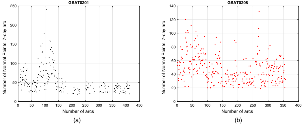
FIG. 27. Number of observations per arc. (a) GSAT0201: normal points per arc. (b) GSAT0208: normal points per arc.
