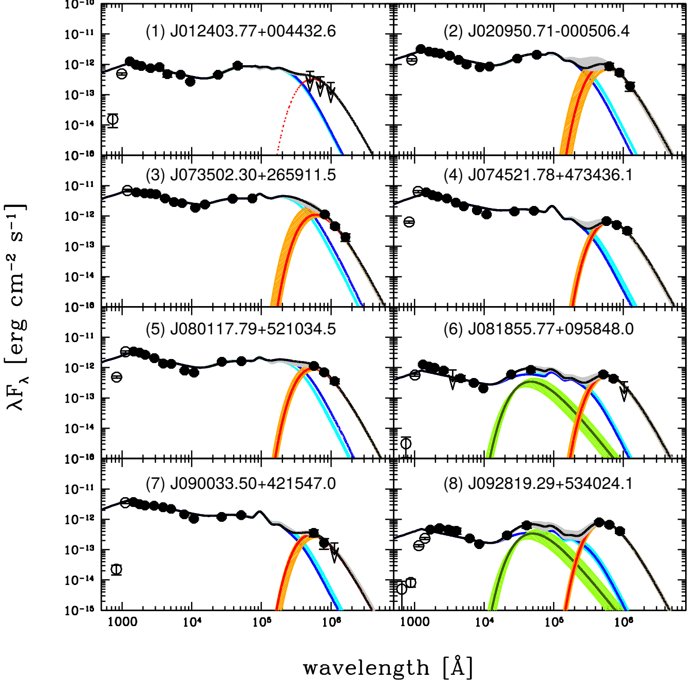
Fig. 5: Resulting rest-frame SED decompositions for half of the sources analyzed (continues in Figure 6). Black circles are the rest-frame photometric points corresponding to the observed bands used to constrain the SED. Black open circles represent the photometric points not included in the fits (at \lambda < 1216 \text{ \AA} due to Ly- \alpha absorption, see the text for more details), while the black arrows correspond to upper limits on the observed flux densities at 1\sigma . Lines (and shaded areas) correspond to the model templates (and the 1\sigma error) found as best-fit solution to describe the photometric points through the \chi^2 minimization: blue is the accretion disk plus torus template (AD+T), red is the Cold dust component (CD) while dark green the NIR excess (NE) when present. Finally, the black line shows the sum off all these contributions. Blue, orange and light green shaded areas correspond to the accretion disk plus torus, the cold dust and the NIR excess templates within 1\sigma of the best-fit template, and light grey shaded area to their sum.
