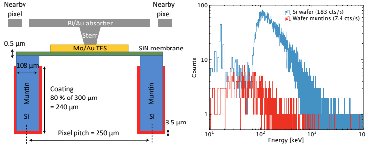
Fig. 1 Left : Schematic of the muntin structure suspending the TES array on a SiN membrane. A coating (typically gold) covers the bottom of each muntin as well as its side up to 80 % (limited by the deposition angle). Figure adapted with permission from [7]. Right : Spectrum of CR induced energy depositions in the Si frame and muntin structure. (Color figure online)
