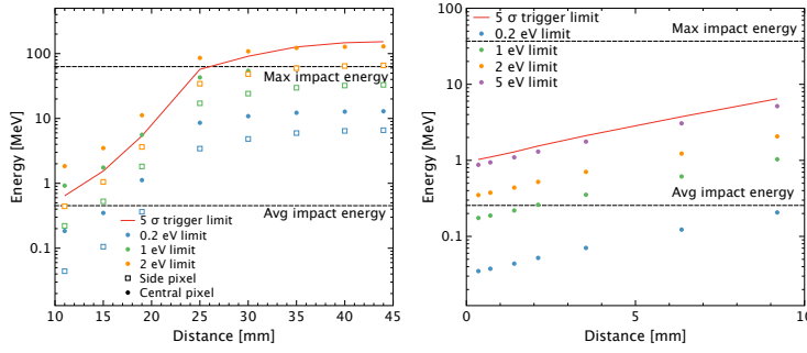
Fig. 7 Comparison between the 5\sigma trigger level and the energy at which a CR deposition can induce different energy offsets. Left: Comparison made for hits in the frame and the baseline heatsinking design. The trigger pixel is assumed to be on the edge of the array. Right: Comparison made for hits in the muntin structure for a pixel and its trigger located at the center of the array. (Color figure online)
