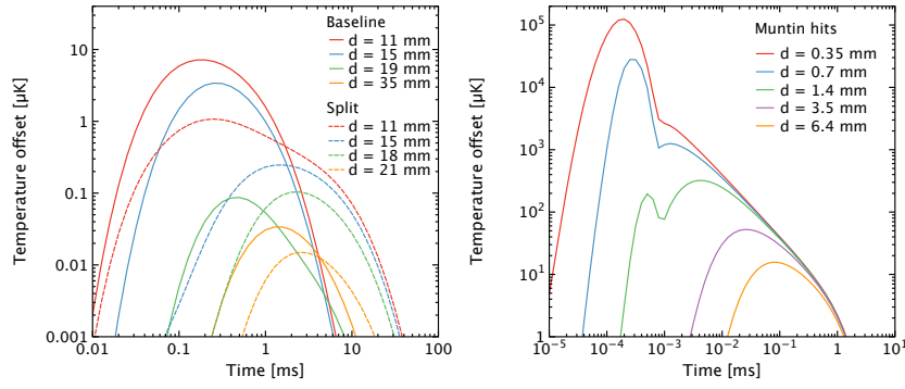
Fig. 3 Simulated temperature pulses measured at the center of the array for CR impacts at varying distances (500 keV). Left: Simulation of impacts in the Si frame for both studied heatsinking configurations. Right: Simulation of impacts in the muntin structure below the pixels. (Color figure online)
