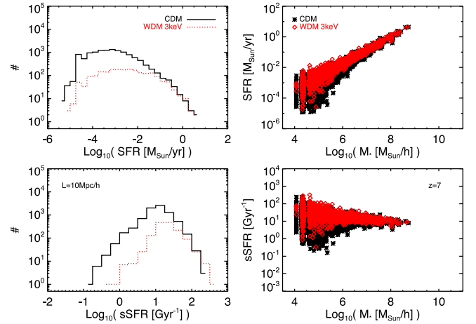
Figure 10. SFR (top left) and sSFR (bottom left) distributions for structures in the CDM and in the WDM scenarios at z = 7 with corresponding M_* -SFR (top right) and M_* -sSFR (bottom right) relations.
