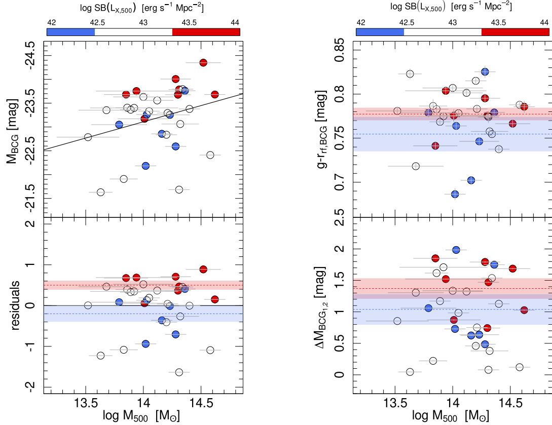
Figure 7. Left panels: absolute magnitude of BCG versus M_{500} (top) with the best fit (black line) and the residuals (bottom). The black line has equation \log M_{BCG} = (-0.68 \pm 0.42) \cdot \log M_{500} - (13.57 \pm 5.93) . Right panels: BCG rest-frame colours (top) and magnitude difference between the BCG and the second brightest cluster galaxy ( \Delta M_{BCG1,2} , bottom) versus M_{500} . Points are colour-coded by SB_X . The magnitude errors are smaller than the symbols.
