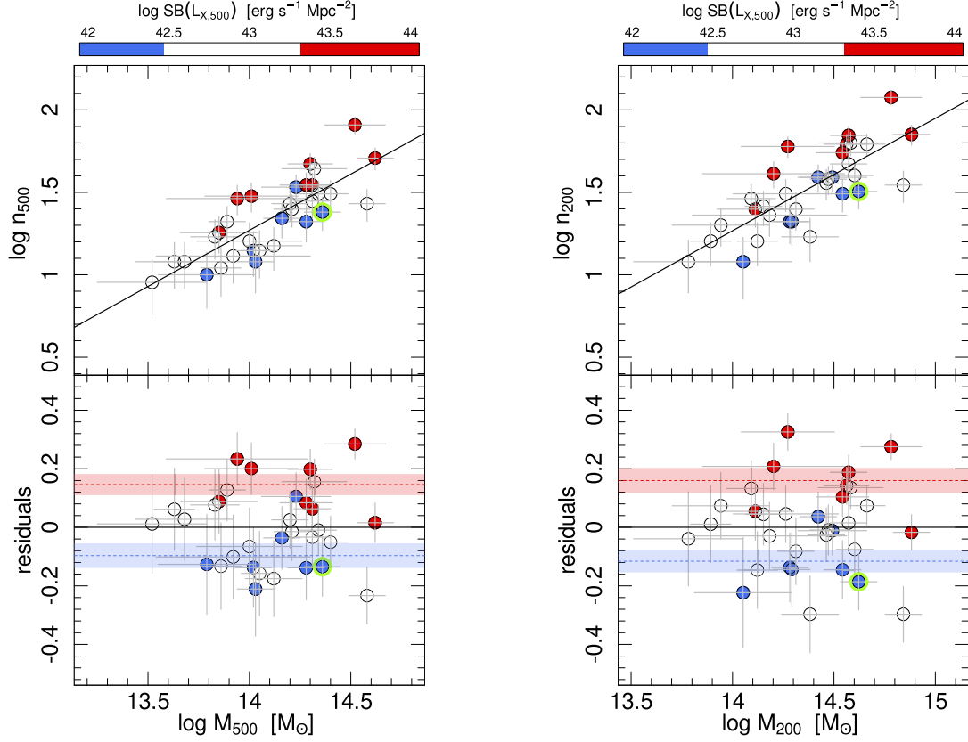
Figure 3. Richness, computed inside r_\Delta (upper panels) versus mass; the fit residuals are plotted in the lower panels. \Delta = 500 at left and \Delta = 200 at right. 1\sigma regions (shaded regions) around the mean values (dashed horizontal lines) are reported for the two populations. The best fit lines have equations \log n_{500} = (0.68 \pm 0.09) \cdot \log M_{500} - (8.27 \pm 1.26) and \log n_{200} = (0.68 \pm 0.1) \cdot \log M_{200} - (8.28 \pm 1.44) . Points are colour-coded by SB_X and CL2015 is marked by a green circle.
