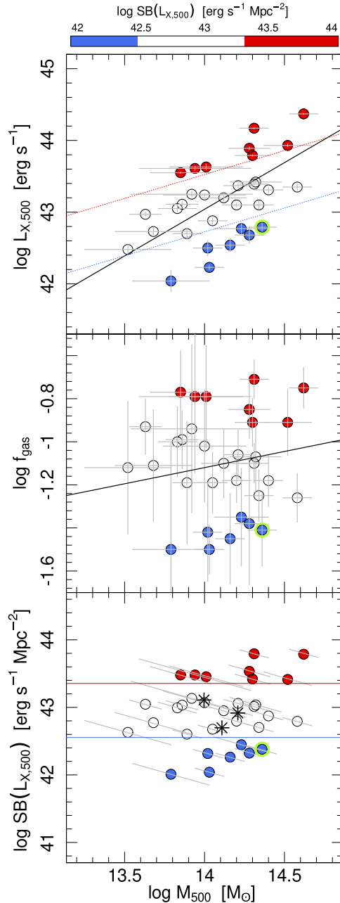
Figure 1. Gas mass and X-ray luminosity versus mass for the XUCS sample. The two upper panels reproduce fig. 4 of Andreon et al. (2017): core-excised luminosity (upper panel) and gas fraction (central panel) versus caustic mass. The solid lines indicate the mean fit for the X-ray luminosity and the gas fraction slopes derived in Andreon et al. (2017). In the lower panel, we plot X-ray surface brightness. Points are colour-coded by SB_X ; we define those above the red line as high- SB_X clusters and those under the blue line as low- SB_X clusters. These red and blue lines are also displayed on the upper panel. The most massive low- SB_X cluster is CL2015, marked by a green circle. The clusters Abell 1631, Abell 76 and Abell 2399, which are low- SB_X clusters in the literature, are overplotted on our sample (starred symbols). Clusters that are gas-poor for their mass are also L_X -faint (for their mass).
