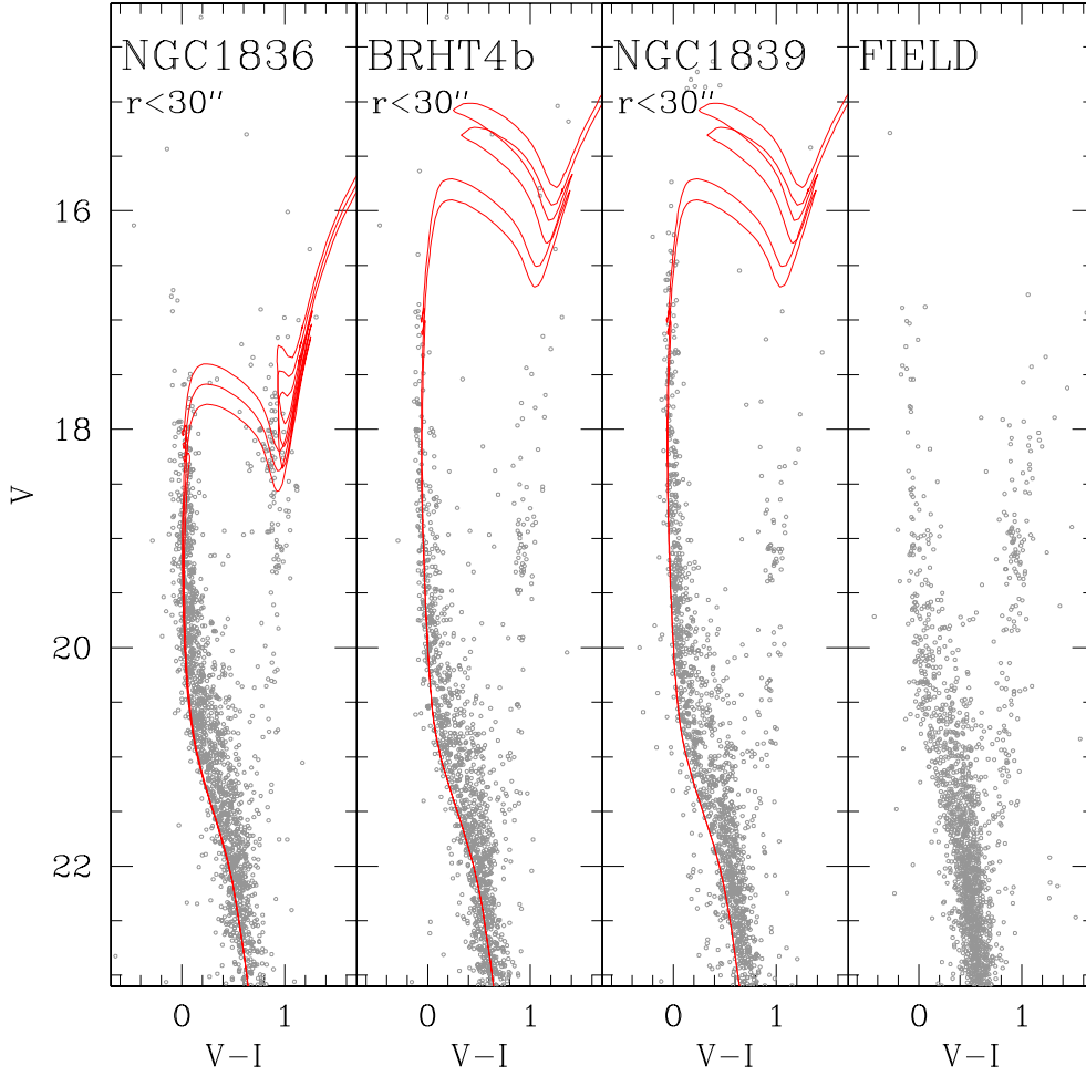
Figure 6. As in Figure 5, but for NGC1836, BRHT4b, NGC1839 and field stars. The area sampled by the field CMD is \sim 2.1 \text{ arcmin}^2 .
