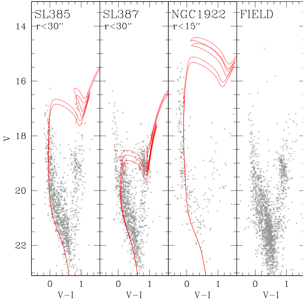
Figure 5. From left to right: color-magnitude diagrams of the clusters SL385, SL387, NGC1922, and of the field stars. The area sampled by the field CMD is \sim 1.3 \text{ arcmin}^2 . As in Figure 4, best-fit isochrones and minimum/maximum age models providing an acceptable fit are shown.
