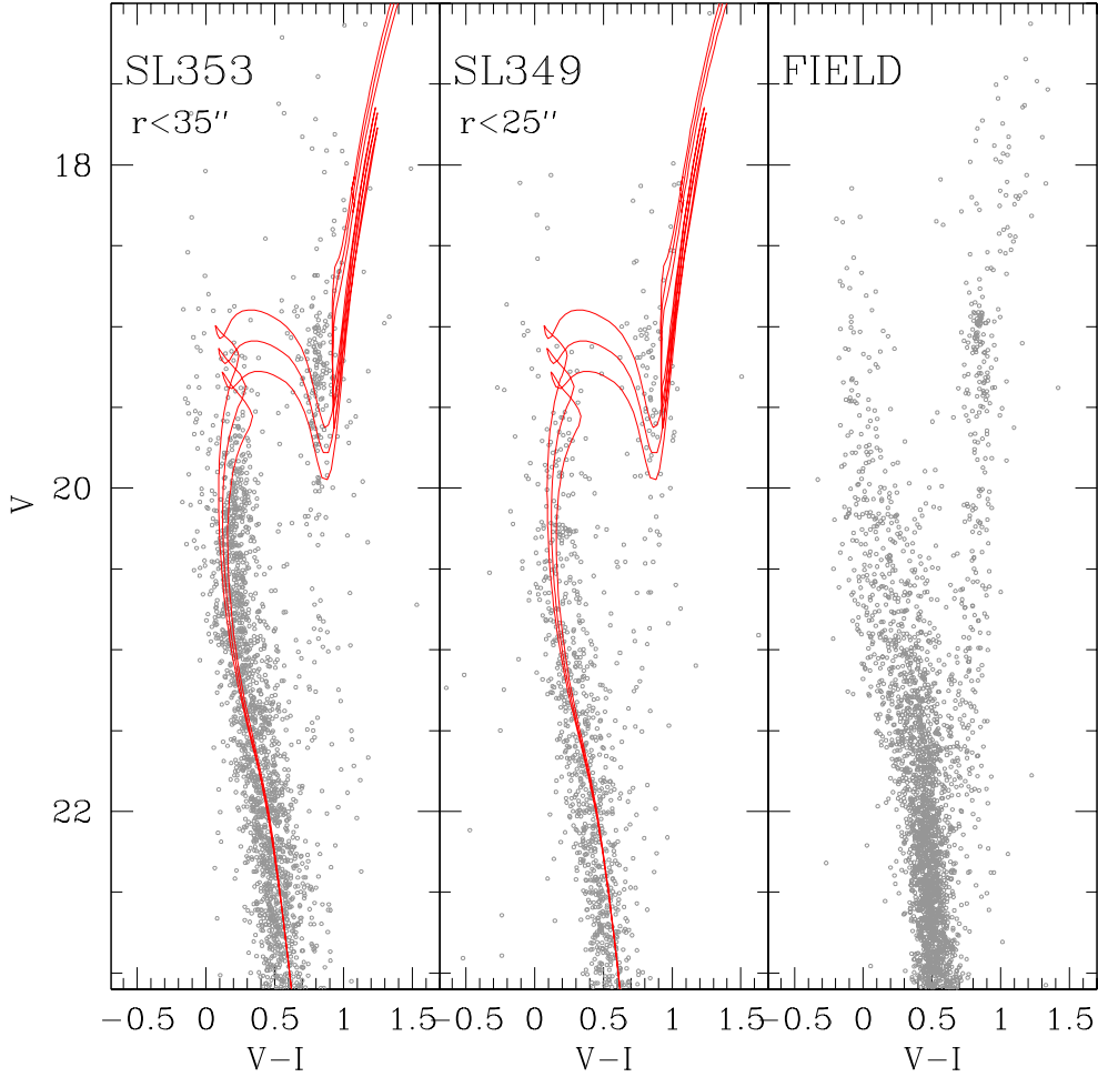
Figure 4. From left to right: color-magnitude diagrams of the clusters SL353 and SL349 and of the field stars. The area sampled by the field CMD is \sim 2.4 arcmin 2 , thus more than 2.5 times the area covered by the CMDs of the two clusters. In the first two panels best-fit isochrones as well as minimum and maximum age models providing an acceptable fit are shown.
