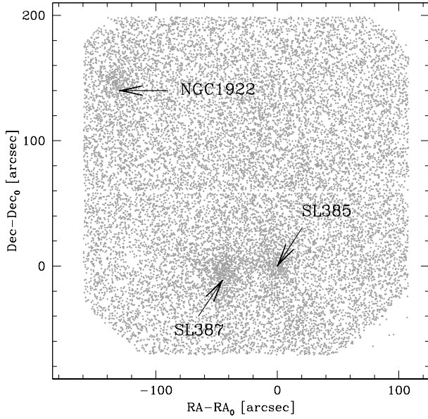
Figure 2. Map of the candidate cluster pair SL387-SL385; the stellar system NGC 1922 is also visible within the field of view. The centre of each cluster is indicated with an arrow.
