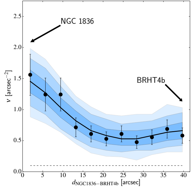
Figure 12. Number density along the line connecting clusters NGC1836 and BRHT4b on the plane of the sky. The format of this figure is the same as Fig. 10.
