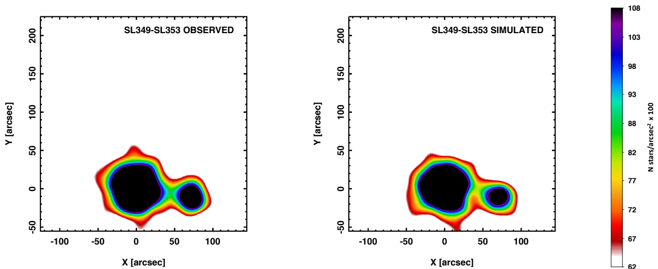
Figure 9. Number density map for the clusters SL353 and SL349. The left panel shows the density map measured from the observations, the right panel the density map obtained from one of our 1000 simulated samples to reproduce this cluster pair. The color code presented in the bar on the right indicates the density scale.
