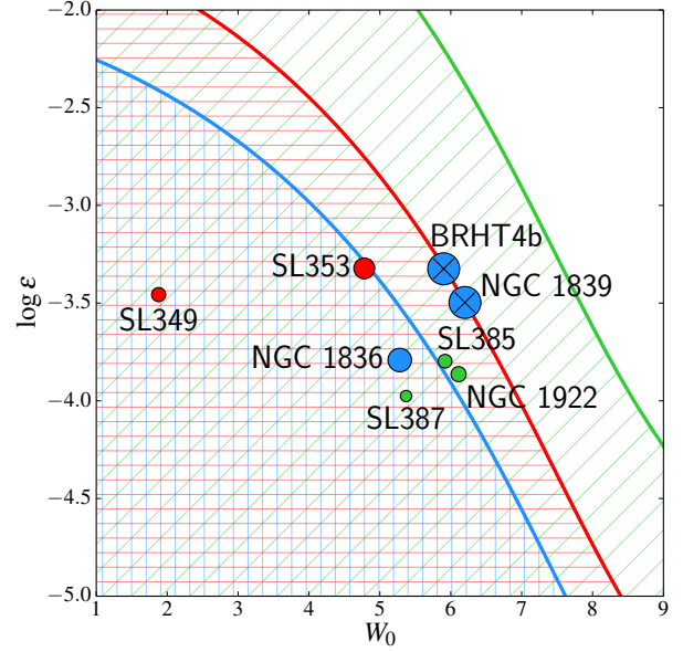
Figure 8. Tidal strength parameter \varepsilon as a function of W_0 . The blue, red and green lines correspond to the critical values of the tidal strength parameter, as a function of W_0 , for clusters located at the galactocentric distance corresponding to parameter values \xi = 0.01, 0.16, 0.55 in a spherical host Plummer potential (for details, see main text). Any cluster located in the shaded region below a given line is underfilling its critical equipotential surface. The clusters in our sample are indicated with circles having the same colors used in Fig. 7 and size representing the value of their filling factor r_t/r_J . Clusters NGC1839 and BRHT4b are marked with a cross because their estimated truncation radius is chosen to be equal to their Jacobi radius.
