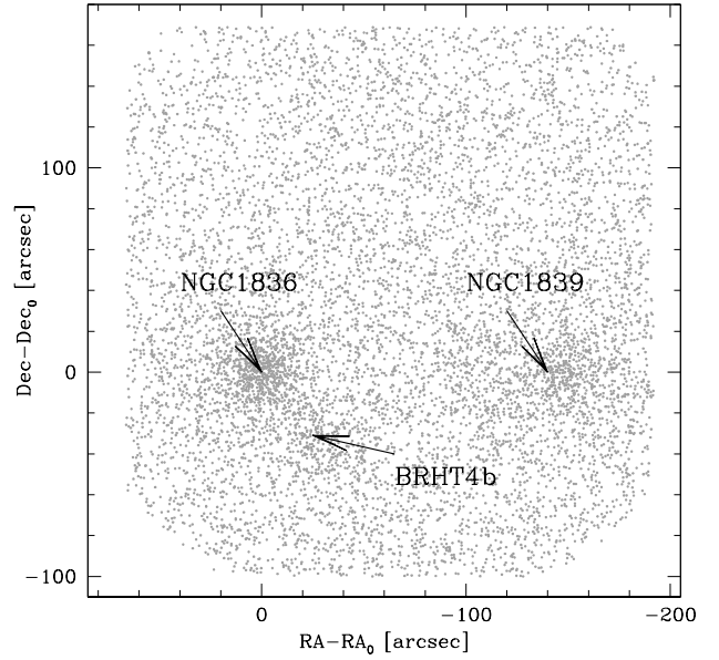
Figure 3. Map of the candidate cluster pair NGC1836-BRHT4b; the stellar system NGC1839 is also visible within the field of view. The centre of each cluster is indicated with an arrow.
