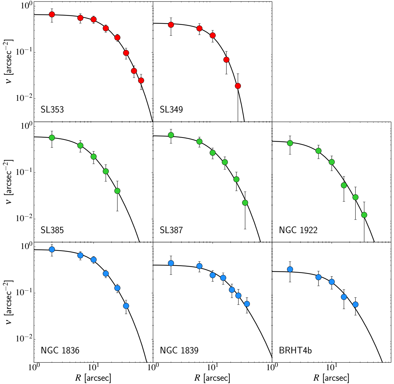
Figure 7. Number density profiles of the clusters in our sample, as indicated by the labels in the panels. Solid lines correspond to the best-fit King (1996) model fits, and the data are indicated with circles. Each row corresponds to a different group of clusters, identified also by the different colors of the points in the panels. For each data-point, vertical error bars are shown. The vertical and horizontal axes span the same range in every panel, to allow a more direct comparison among the clusters.
