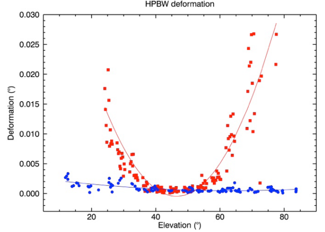
Fig. 15. Beam deformation, with respect to the ideal beam size, versus elevation. Squares: with fixed optics. Circles: with active surface and subreflector in tracking mode ( \sigma = 2.25 arcsec).
