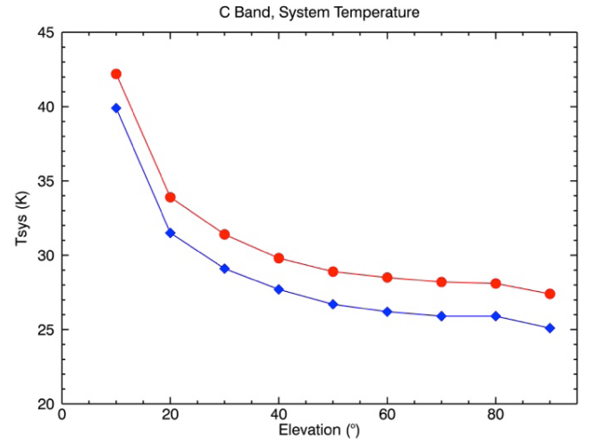
Fig. 8. Tsyst measured in the band 6.7–7.7 GHz. Circles: LCP. Diamonds: RCP.
