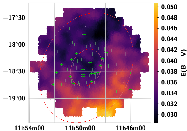
Figure 3. Reddening map, E(B-V)_{\text{SFD}} , in the Crater II region from Schlegel et al. (1998) . Green asterisks mark the location of the RR Lyrae stars identified in this work. Red lines represent the best fitted 1\sigma and 3\sigma ellipses to the population of RR Lyrae stars (see § 4.5). To obtain the extinction A_g and A_i we used the coefficients derived by Schlafly & Finkbeiner (2011) .
