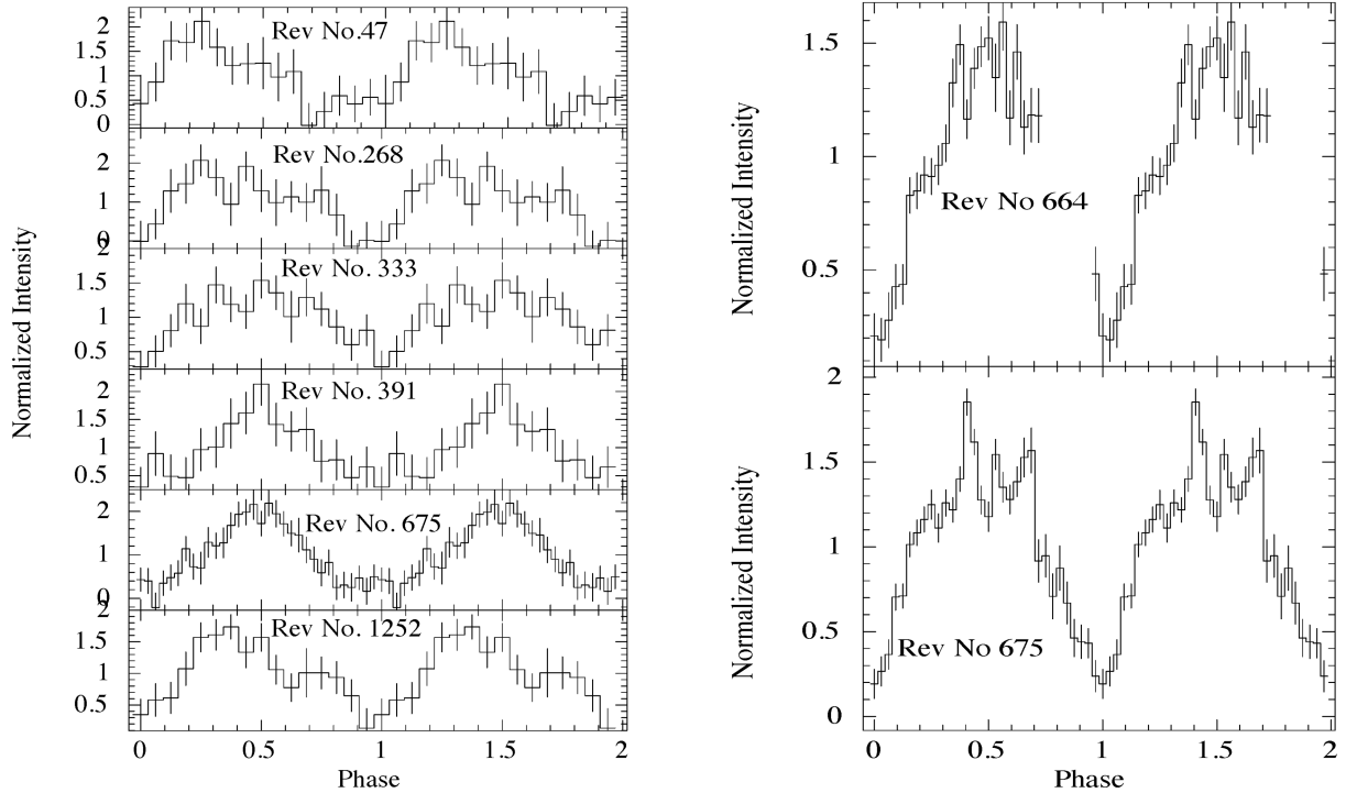
Figure 7. Left: pulse profiles extracted from the IBIS/ISGRI data (20–40 keV). Right: pulse profile extracted from the JEM-X data (3–35 keV). In both panels, the epoch chosen for the folding is arbitrary.
