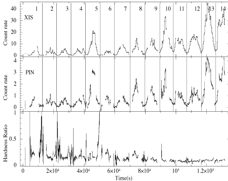
Figure 1. Background subtracted Suzaku light curves of 4U 0114+65. The time bin is 300 s. The upper and middle panels show the XIS and HXD-PIN data, respectively. The hardness ratio of the XIS and HXD-PIN data is reported in the bottom panel. The start time of the light curves is 55763.4805 MJD.
