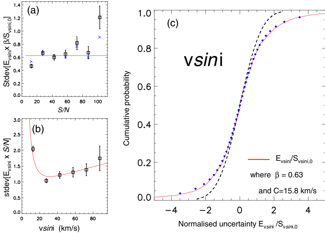
Fig. 4. Analysis of the empirical uncertainty for short-term repeat observations of v \sin i using order-sorting filter HR15N. Plot a ) shows the variation of E_{v \sin i} \times (S/N)/([v \sin i]/C)^2/(1 + ([v \sin i]/C)^2)^{5/4} with S/N . The horizontal line indicates the value of parameter \beta in Eq. (3) fitted to the full dataset. Blue crosses show the estimated values \beta as a function of S/N corrected for the measured variation of \beta with T_{\text{eff}} (see Sect. 4.4 and Table 3). Plot b ) shows the variation of E_{v \sin i} \times S/N with v \sin i . The solid line shows the relationship predicted using the theoretical value of C and the value of \beta from plot a ). In plots a ) and b ) the y -axis shows an estimate of the standard deviation based on the MAD divided by 0.82 (for \nu = 2 , see Sect. 3.3). Plot c ) shows the cumulative probability distribution (CDF) of the normalised uncertainty in v \sin i for short-term repeats. The red solid line shows results for measured data, the dashed line shows the cumulative distribution of a Gaussian with unit dispersion, and the diamond symbols show the cumulative distribution function for a Student's t -distribution with \nu = 2 .
