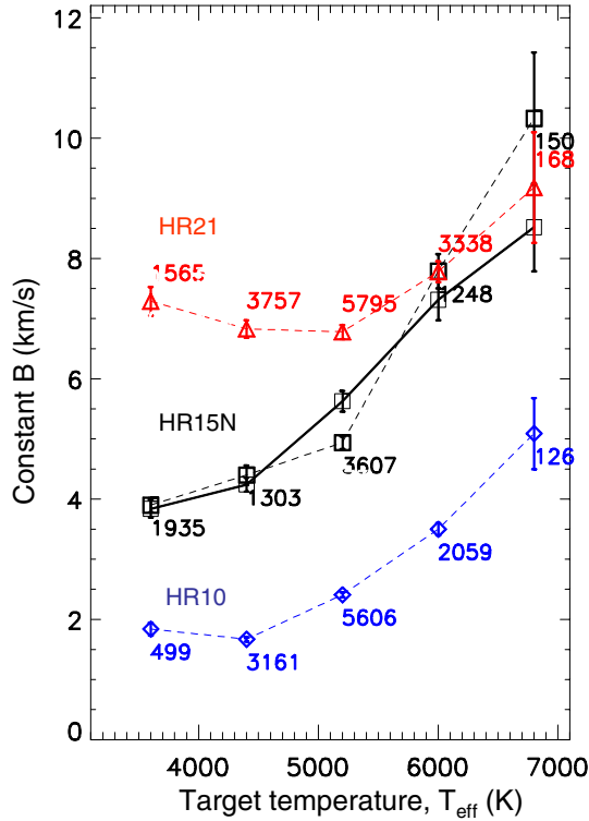
Fig. 5. Variation of parameter B of the scaling function for uncertainty in RV ( S_{RV} ) with effective temperature. The solid line shows results for filter HR15N as a function of T_{eff} (see Sect. 4.1). Dashed lines show results for filters HR10, HR15N and HR21 as a function of the temperature of the template spectrum fitted in the CASU pipeline (see Sect. 2.3). Numbers equal the sample size per bin.
