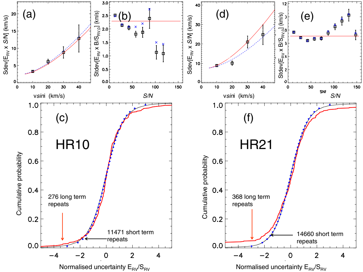
Fig. 10. Analysis of the empirical uncertainty for short term repeat observations of RV using filter HR10 and HR21. Plots a) and d) show the variation of E_{RV} with v \sin i . Red lines show the curves predicted using the model value of C (see Eq. (A.4)). The dashed lines show the curves predicted using values of B and C fitted to the binned data. Plots b) and e) show the variation in the estimated value of parameter B in Eq. (1) with S/N . Red lines show values of B fitted to the full dataset for each filter. Blue crosses show the estimated values B as a function of S/N corrected for the measured variation of B with T_{\text{eff}} (see Table 3). Plots c) and f) show the normalised uncertainty for short term repeats and long term repeats. The black curve shows the CDF for short-term repeats. The red line shows the CDF for long-term repeats. Blue diamonds show a Student's t-distribution with \nu = 6 , which matches the distribution for short-term repeats well.
