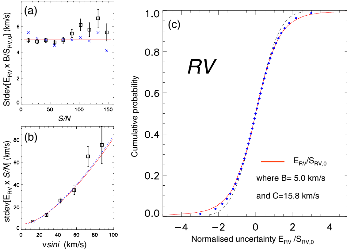
Fig. 3. Analysis of the empirical uncertainty for short-term repeat observations of RV using filter HR15N. The solid line in plot a ) shows the variation of E_{\text{RV}} \times (S/N)/(1 + ([v \sin i]/C)^2)^{3/4} with S/N . The horizontal line indicates the value of parameter B in Eq. (1) fitted to the full dataset. Blue crosses show the estimated values B as a function of S/N corrected for the measured variation of B with T_{\text{eff}} (see Sect. 4.1 and Table 3). Plot b ) shows the variation of E_{\text{RV}} \times S/N with v \sin i . The solid line shows the relationship predicted using the theoretical value of C and the value of B from plot a ). The dashed line shows a curve of similar functional form using parameters B and C fitted to the binned data. In plots a ) and b ) the y -axis shows an estimate of the standard deviation based on the MAD divided by 0.72 (see Sect. 3.2). Plot c ) shows the cumulative probability distribution (CDF) of the normalised uncertainty in RV for short-term repeats. The red solid line shows results for measured data, the dashed line shows the cumulative distribution of a Gaussian with unit dispersion, and the diamond symbols show the cumulative distribution function for a Student's t -distribution with \nu = 6 .
