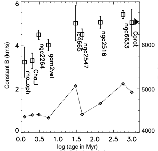
Fig. 7. Variation of parameter B of the scaling function for uncertainty in RV ( S_{RV} ) with target age for observations with order-sorting filter HR15N. Square symbols show the value of B for targets identified as possible cluster members from their RV versus the nominal age of the cluster (see Table 1). No selection by RV is made for NGC 6633 or COROT and we assume the stars have mean ages > 1 Gyr. The dotted line indicates the median value of T_{eff} (right hand axis values) for members identified in each cluster.
