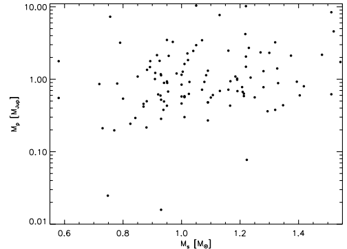
Fig. 9. Planetary mass, in Jupiter mass, against the mass of the host, in Sun mass for the systems considered in this analysis.
