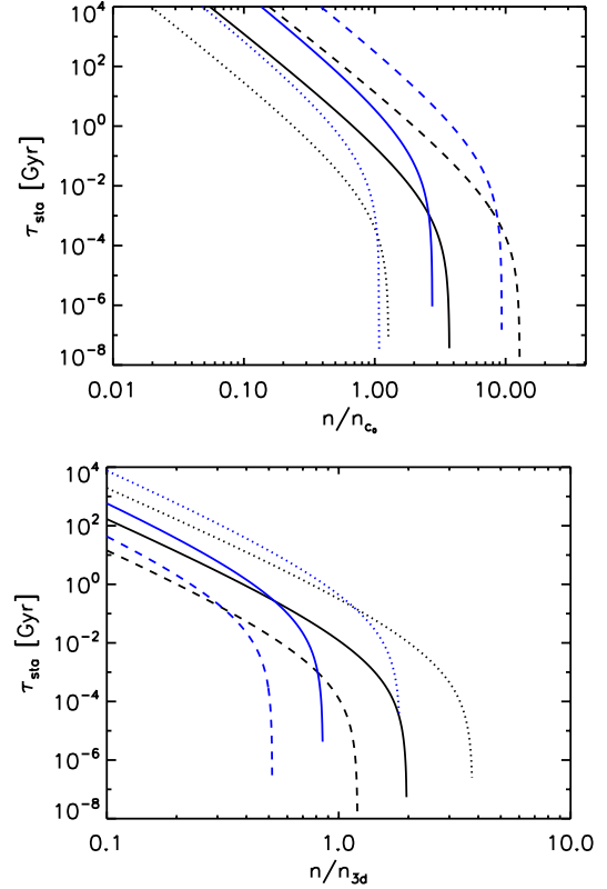
Fig. 6. Top: estimates of the maximum possible duration of the stationary state \tau_{\text{sta}} as a function of the orbital mean motion in units of the critical mean motion n_{c_0} . The computations were done for a G-type star (black) or F-type star (blue) and planetary masses of 0.1 (dashed), 1 (solid), and 10 (dotted) Jupiter masses. We used Q' = 10^7 for both G- and F-type stars, while the magnetic braking coefficient \alpha_{\text{mb}} is reduced by a factor of ten for F-type stars (see text). Bottom: the same, but the orbital mean motion is in units of n_{3d} = 2\pi/(3 \text{ days}) , hence independent of planetary and stellar mass.
