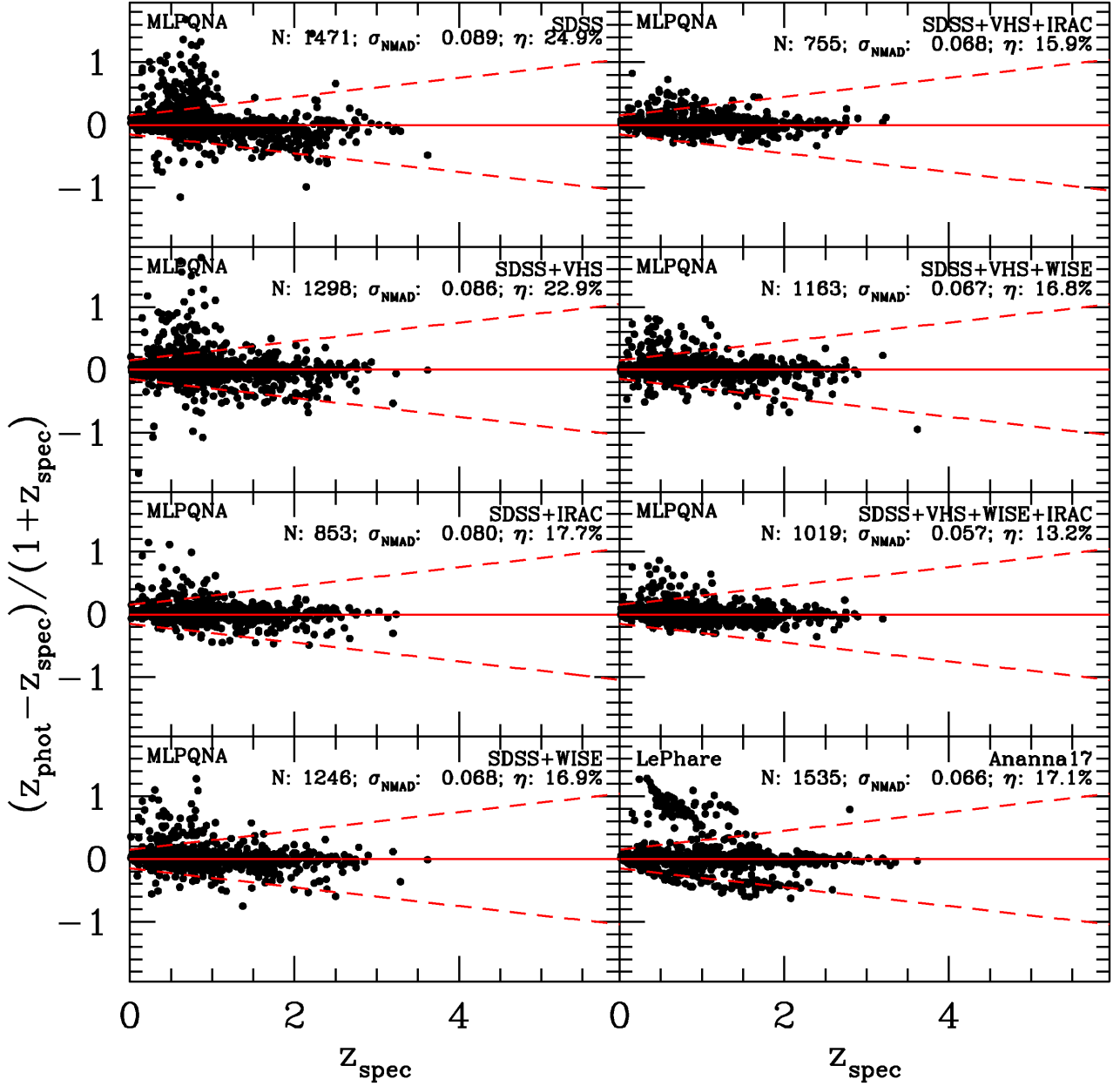
Figure 5. Comparison between spectroscopic redshift and photo- z for the sources cut at the eROSITA flux and divided on the basis of available photometric points. For comparison, the result from A17 is reported in the lower right panel of the figure. By comparing the accuracy and the fraction of outliers in every panel with the corresponding row in Table 8, we see that computing photo- z using only SDSS for bright X-ray sources is not recommended.
