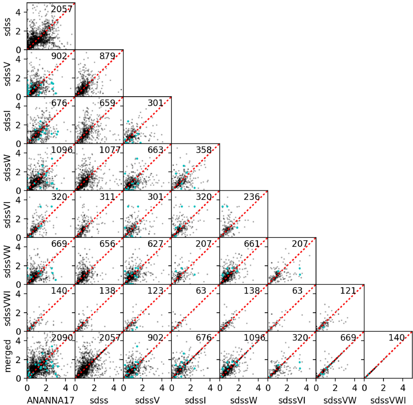
Figure A2. Comparison between photo- z computed via SED fitting (A17) and MLPQNA for the sample for which spectroscopic information is not available. The cyan points indicate the sources for which the redshift could be computed only after considering supplementary photometry in addition to SDSS.
