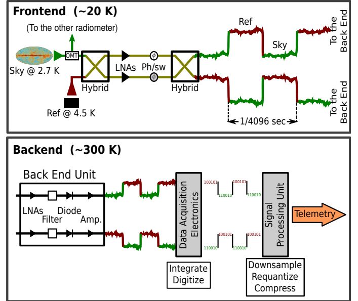
Fig. 1. Schematics of an LFI radiometer taken from Cal13. The two linearized polarization components are separated by an orthomode transducer (OMT), and each of them enters a twin radiometer, only one of which is shown in the figure. A first amplification stage is provided in the cold (20 K) focal plane, where the signal is combined with a reference signal originating in a thermally stable 4.5-K thermal load. The radio frequency signal is then propagated through a set of composite waveguides to the warm (300 K) backend, where it is further amplified and filtered, and finally converted into a sequence of digitized numbers by an analogue-to-digital converter. The numbers are then compressed into packets and sent to Earth.
