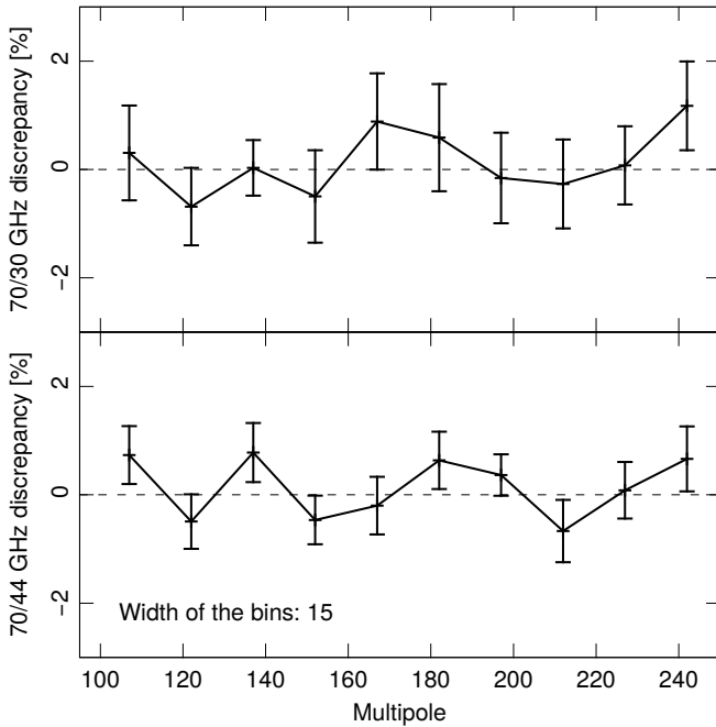
Fig. 11. Estimate of \Delta_{\ell}^{70 \text{ GHz, other}} (Eq. (45)), which quantifies the discrepancy between the level of the 70 GHz power spectrum and the level of another map. Top : comparison between the 70 GHz map and the 30 GHz map in the range of multipoles 100 \leq \ell \leq 250 . The error bars show the rms of the ratio within each bin of width 15. Bottom : the same comparison done between the 70 GHz map and the 44 GHz map. A 60% mask was applied before computing the spectra.
