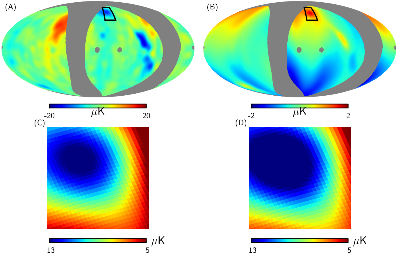
Fig. 12. Difference in the application of the full 4\pi beam model versus the pencil beam approximation. Panel A): difference between survey 1 and survey 2 for a 30 GHz radiometer (LFI-27S) with the 4\pi model, smoothed to 15^\circ . We do not show the same difference with pencil beam approximation, because it would appear indistinguishable from the 4\pi map. Panel B): double difference between the 4\pi 1-2 survey difference map in panel A and the pencil difference map (not shown here). This map shows what changes when one drops the pencil approximation and uses the full shape of the beam in the calibration. Panel C): zoom on the blue spot visible at the top of the map in panel A). Panel D): same zoom for the pencil approximation map. The comparison between panels C) and D) shows that the 4\pi calibration produces better results.
