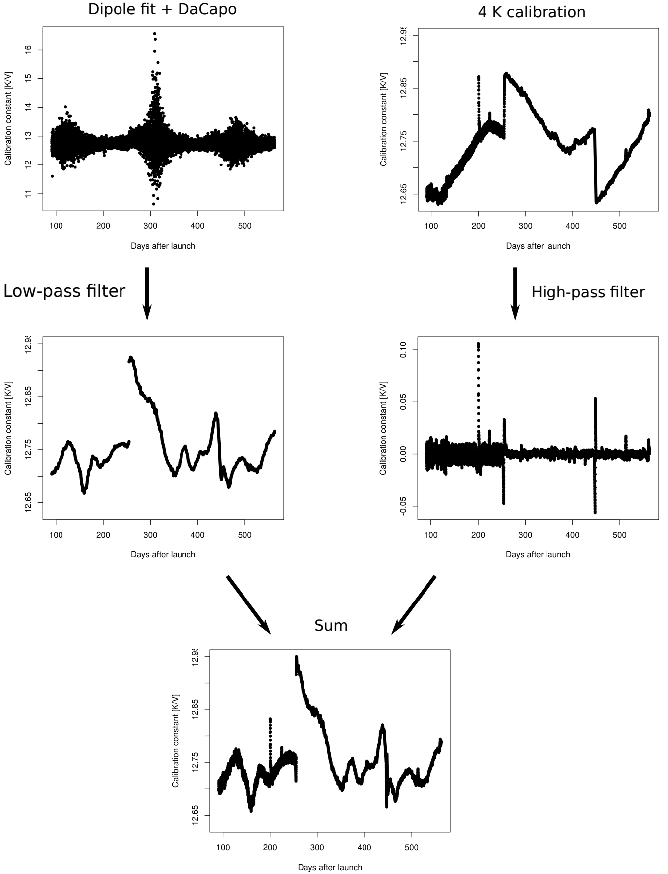
Fig. 5. Visual representation of the algorithms used to filter the calibration constants produced by DaCapo ( top left plot ; see Sect. 4). The example in the figure refers to radiometer LFI-27M (30 GHz) and only shows the first part of the data (roughly three surveys).
