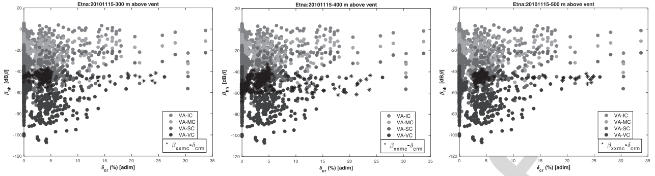
Fig. 3. Lidar data collected during the November 15, 2010 ash emission at Mt. Etna in Italy. Superimposition between measured (dark dots) and simulated backscatter coefficient \beta_{hh} (in dB) and cross-polarization ratio \delta_{cr} (in %) at (Left) 300, (Middle) 400, and (Right) 500 m of altitude above Etna summit craters, respectively. Different color identifies different concentration classes (IC in magenta, MC in green, SC in red, and VC in blue), all for the VA class.
