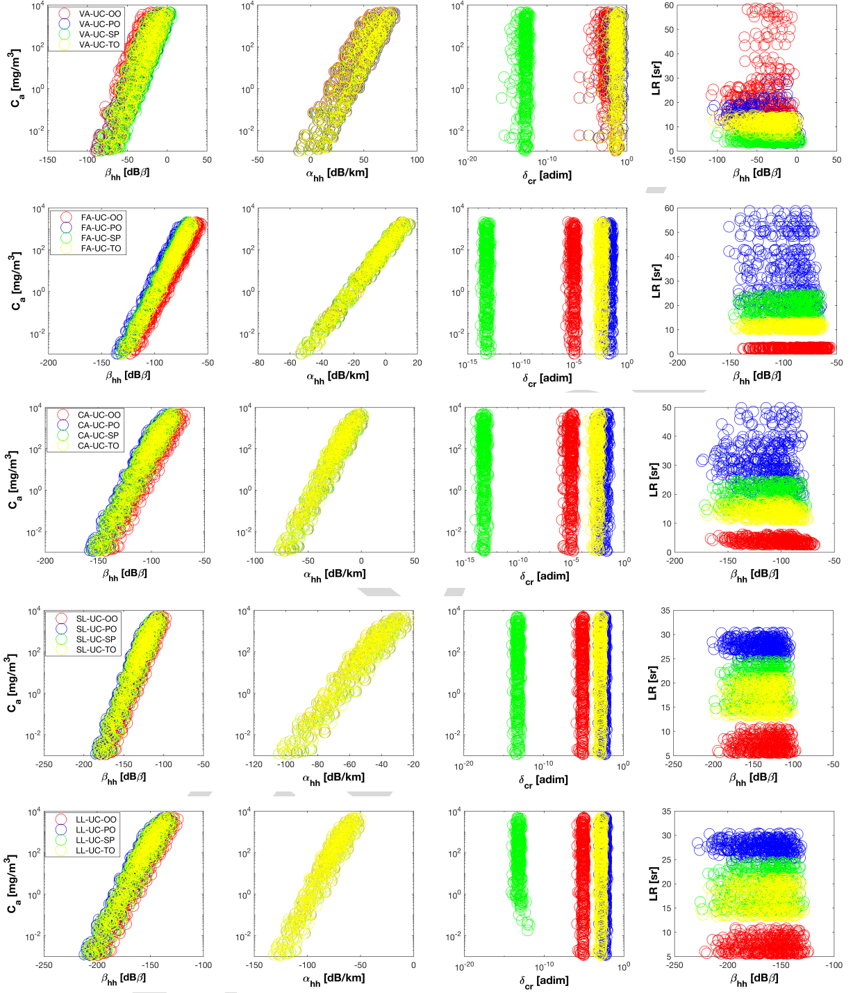
Fig. 2. Numerical results of the HAPRESS simulations at 532-nm wavelength (VIS). Correlation between ash mass concentration C_a ( \text{mg}/\text{m}^3 ) and both backscatter (in \text{dB}/\beta ) and extinction coefficients (in \text{dB}/\text{km} ) in the top panels (left and right panels, respectively) and between LidarLR and backscatter and between ash mass concentration C_a ( \text{mg}/\text{m}^3 ) and cross-polarization in the bottom panels (left and right panels, respectively), for each ash class VA, FA, CA, SL, and LL ( 2 \times 2 panels), for different orientations (OO, PO, SP, and TO) and for uniform concentration (UC) (between 1 and 10^7 \mu\text{g}/\text{m}^3 ). See text and Table I for details.
