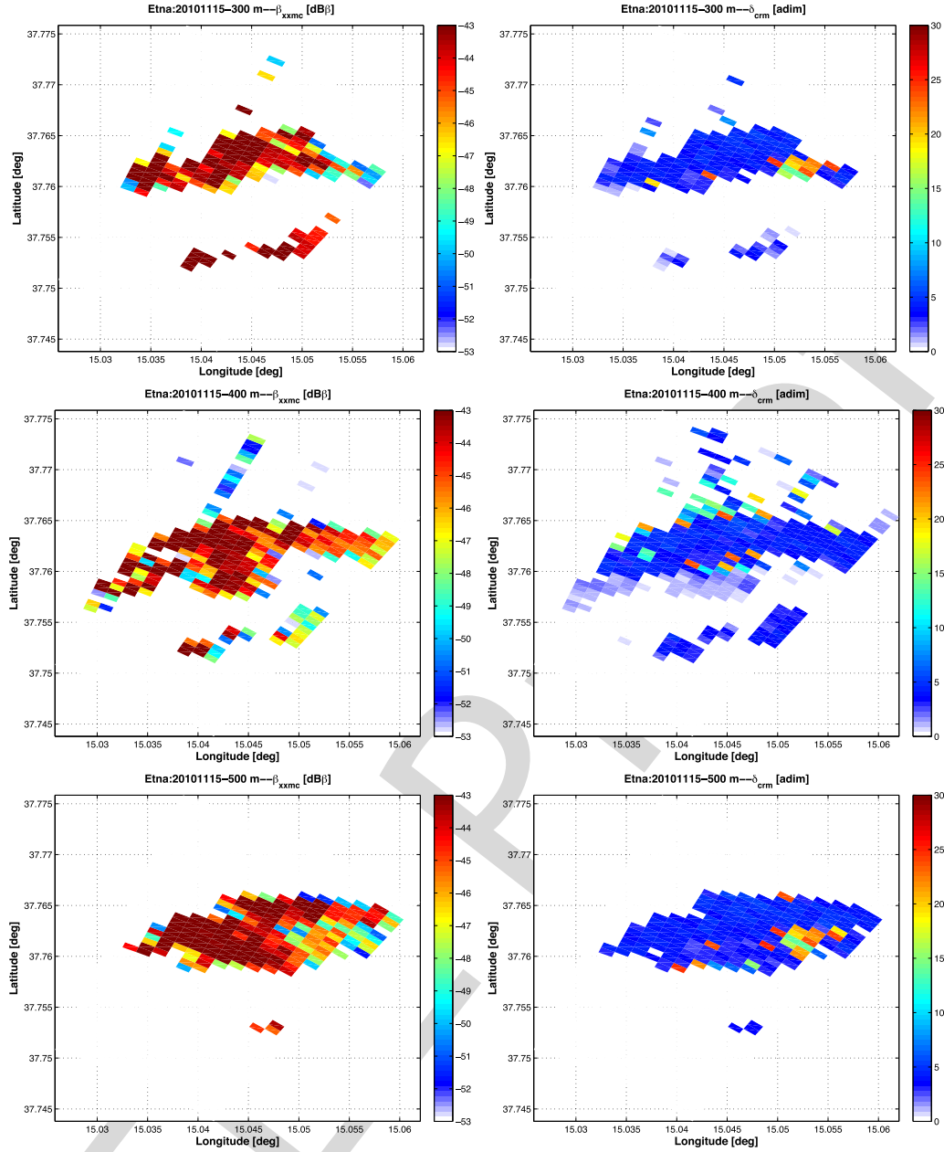
Fig. 4. Lidar data collected during the November 15, 2010 ash emission at Mt. Etna in Italy. Maps of the measured backscatter coefficient (in dB \beta ) and linear volumetric depolarization (in %), left and right panels, respectively, at each elevation (300, 400, and 500 m) above the Etna summit craters.
