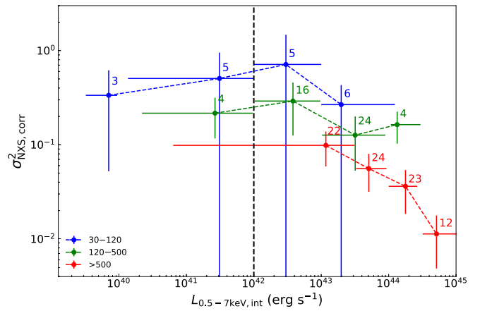
Figure 10. Medians of \sigma^2_{\text{NXS,corr}} vs. L_{0.5-7\text{keV,int}} in different net-count bins for the 148 variable AGNs (136 variable AGNs and 12 variability-selected AGN candidates). The blue, green, and red points represent the net-count bins of 30–120, 120–500, and >500, respectively. The horizontal error bars indicate the luminosity bin width, and the vertical error bars are the median of uncertainties on \sigma^2_{\text{NXS,corr}} . The labels are the number of variable AGNs in each luminosity bin. The black dashed line is the typical LLAGN luminosity demarcation line ( L_{0.5-7\text{keV,int}} \lesssim 10^{42} \text{ erg s}^{-1} for LLAGNs).
