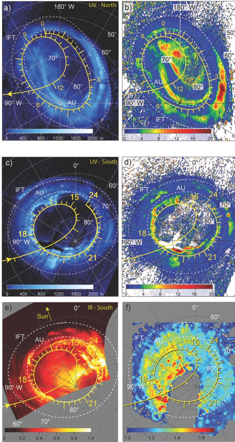
Fig. 6. Orthographic polar projections at the 1 bar level of the ultraviolet (panels a-d) and infrared (e-f) auroral emissions, comparing auroral intensities (left column) and spectral color ratios (right column) with the model auroral oval (innermost dashed oval) and Io footprint (outer dashed circle) computed using the VIP4 model internal field and a model magnetodisc. The
