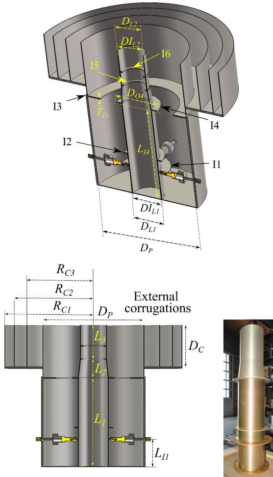
FIGURE 4. Section view and 3D view (CST Studio Suite Model) of the coaxial L-P feed and OMJ.
