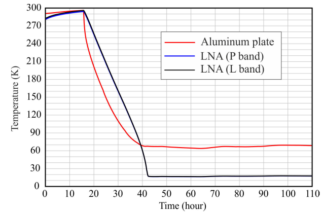
FIGURE 17. Cooldown curve of the coaxial receiver.
