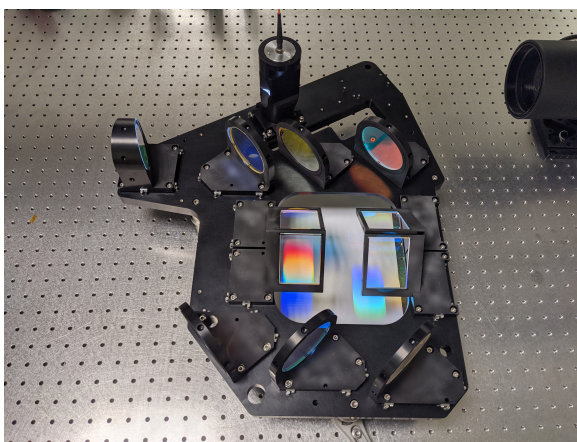
Figure 2. Left: Layout of the feed. A: Folding mirror; B: Off-axis parabola collimator; C/D/G: Dichroic mirrors dividing u + g from r + i , r from i , and u from g , respectively; E/F/H: Dielectric mirrors reflecting i , u + g , and g , respectively; I: gratings. Right: the as-built feed illuminated with a white light source.
