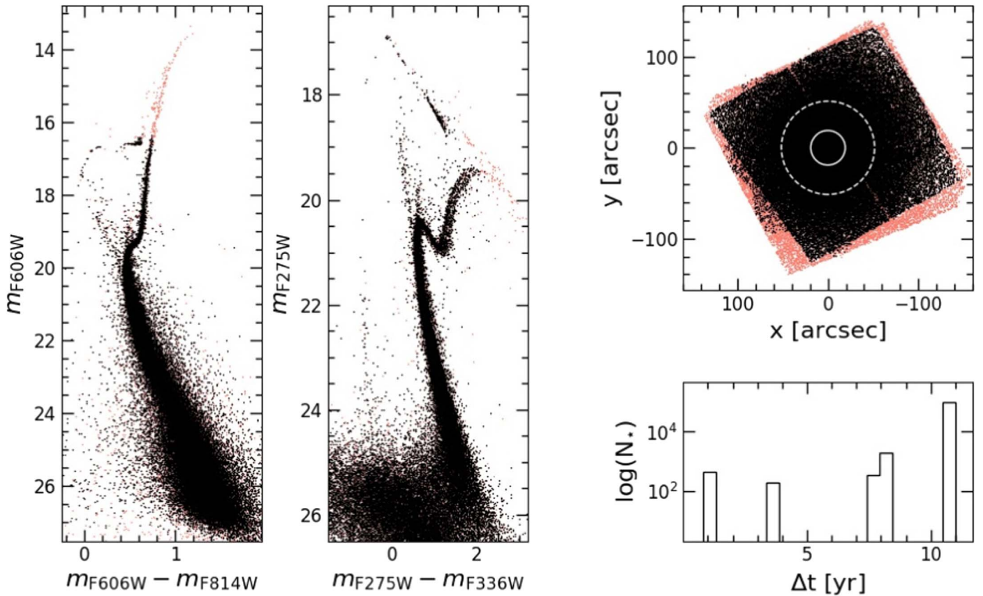
Figure 1. Overview of the NGC 1261 catalog obtained in this work. In all panels, the red dots refer to the complete photometric catalog, while the black dots are stars for which we also have a PM measurement. In the left and central panels, we show the optical ( m_{F606W} vs. m_{F606W} - m_{F814W} ) and UV-blue ( m_{F275W} vs. m_{F275W} - m_{F336W} ) CMDs of NGC 1261. In these plots, we show all stars, regardless of their astrophotometric quality. The scattered cloud of points in the bottom left region of the UV-blue CMD is composed of stars that are measured in the F606W and/or F814W bands but are too faint to be detected in the UV-blue bands. In spite of this, the software forces a fit, which results in an unreliable magnitude estimate that makes the star appear in this region of the CMD. In the upper right panel, we show the FOV covered by our data set, with the center of the cluster (obtained as in Section 3) placed at (0, 0) and the projected positions of each star with respect to the center plotted along the x - and y -axes. North is up and east is to the left. In this panel, we also show r_c and r_h as solid and dashed white circles, respectively, as obtained in Section 3. In the lower right panel, we show the number of objects (in a logarithmic scale) in our PM catalog, as a function of the temporal baseline of the observations used to measure them.
