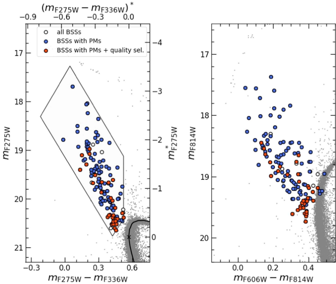
Figure 7. Left panel: UV CMD of the BSS region of NGC 1261. The shaded box with black contours is the BSS selection box (see the text for details). The axis of the n-CMD (i.e., a CMD with color and magnitude rigidly shifted to locate the TO at (0, 0)) is reported in the right and top axes. The isochrone and the relative TO point are shown as a black curve and a black cross, respectively. All of the stars that fall within the selection box in this CMD are selected as BSSs (black empty circles). We show as blue solid circles all of the BSSs that have a measured PM, and in red, the BSSs with a measured PM that also pass the selection criteria described in Section 4.1. Right panel: optical m_{F814W} vs. m_{F606W} - m_{F814W} CMD, with the UV-selected BSSs shown with the same color code adopted in the left panel.
