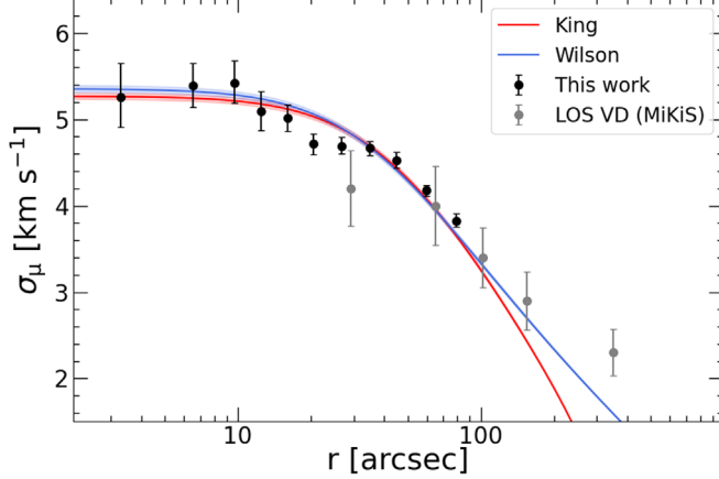
Figure 5. Global velocity dispersion profile of NGC 1261. The measurements in the plane of the sky, obtained from HST PMs are plotted as black circles, while the gray circles correspond to the LOS velocity dispersion profile from Ferraro et al. (2018b). The best-fit King and Wilson profiles are shown as red and blue lines, respectively. The shaded areas around the two best-fit profiles represent the uncertainty on the central velocity dispersion (see the text for details on the fitting procedure).
