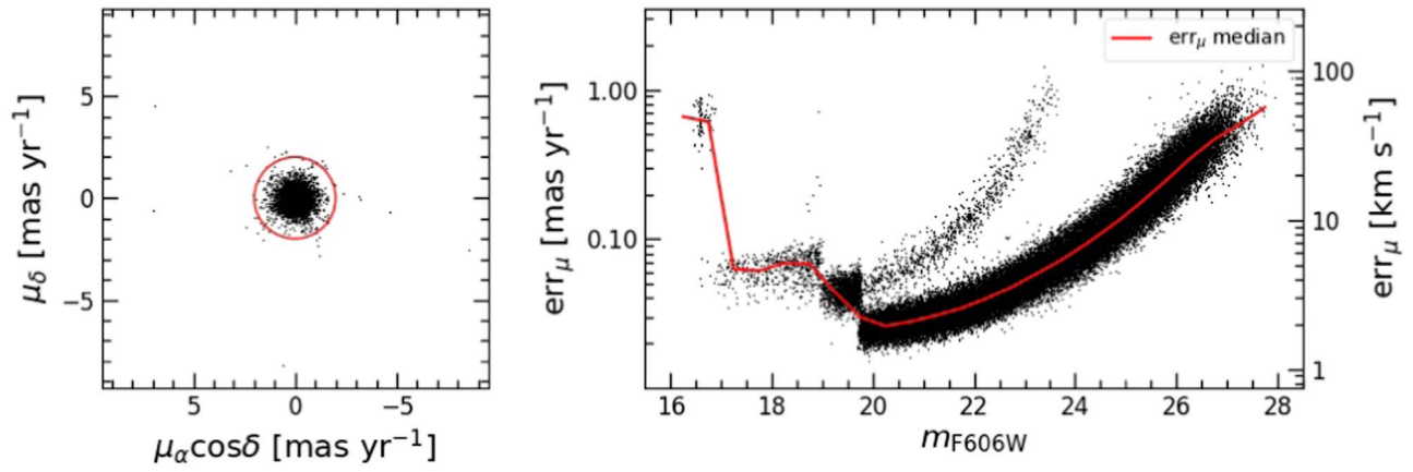
Figure 3. Left panel: VPD of the stars satisfying criteria (i)–(vii), see the text for details. The red circle corresponds to 2 mas yr -1 , marking the threshold adopted to reject non-cluster members (note, however, the very low level of field contamination). Right panel: 1D PM error as a function of the F606W magnitude for the stars satisfying criteria (i)–(vii). The multiple sequences and discontinuities are due to the different temporal baselines and number of images used to compute the PMs in our project. The red line is the median value of \text{err}_\mu , measured in magnitude bins 0.5 mag wide.
