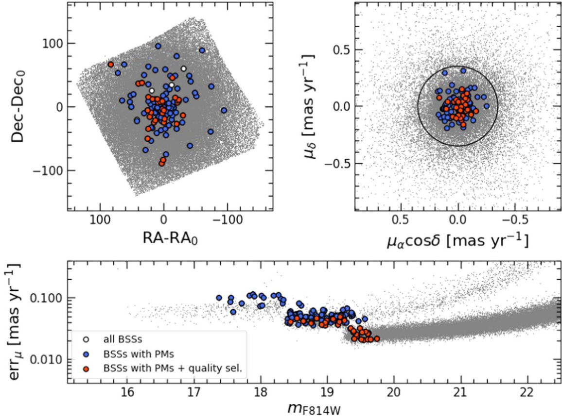
Figure 8. Top left panel: map of the FOV analyzed in this work. We report in gray all of the stars from the photometric catalog and the selected BSSs as large circles. Here and in the other panels, we use for BSSs the same color code adopted in Figure 7, i.e., empty circles for the complete sample of BSSs, blue circles for BSSs with a PM measurement, and red circles for BSSs with a PM measurement that pass the kinematic selection criteria described in Section 4.1. As expected, BSSs are placed preferentially in the central region of the cluster. Top right panel: a zoomed version of the VPD shown in the left panel of Figure 3. We show in gray the stars satisfying criteria (i)–(vii) (see Section 4.1). The black circle corresponds to three times the standard deviation of the PM distribution for stars in a magnitude range comparable to BSSs ( 17 < m_{F814W} < 20 ). Although this value represents a reasonable threshold to separate member BSSs from field contaminants, all BSSs (blue and red circles) fall within this threshold value. Bottom panel: 1D PM error with respect to the F814W magnitude. Clearly, BSS PM errors become larger for increasing stellar luminosity. This is due to the effect of saturation, occurring at different magnitudes for different data sets and, thus, reducing the total time baseline and/or the number of available exposures that can be used to compute PMs.
