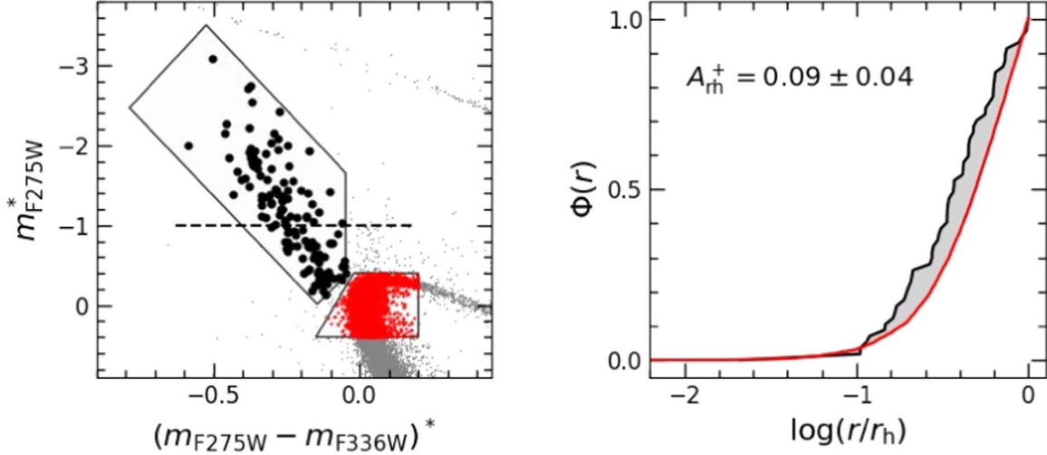
Figure 9. Left panel: n-CMD of NGC 1261. We show as black circles the selected BSSs. The black dashed line corresponds to the magnitude threshold adopted to measure A_m^+ (only BSSs brighter than this magnitude have been used). The red dots are the MS-TO stars used as a reference population. Right panel: cumulative radial distribution of BSSs (black line) and MS-TO reference population (red line). The resulting value of A_m^+ is labeled within the panel.
