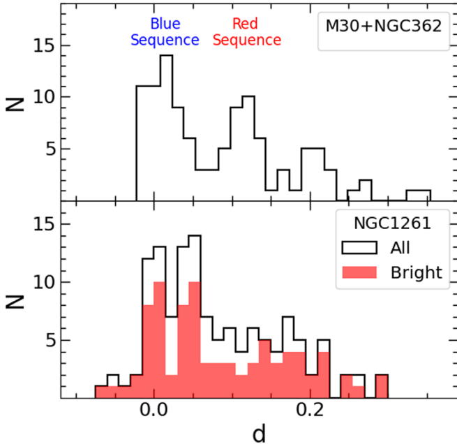
Figure 11. Histograms of the distances of BSSs in M30+NGC 362 (top panel) and in NGC 1261 (bottom panel). The red histogram in the bottom panel shows the distribution of BSSs brighter than m_{F275W} = 20 .
