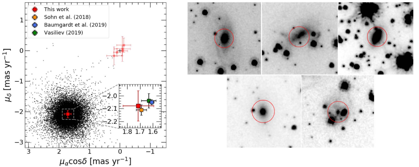
Figure 6. Left panel: VPD of the absolute proper motions. The light red squares are the PMs of the five background galaxies found by visually inspecting the images. The cluster absolute proper motion is marked as a dark red square. In the inset, we zoom in around the cluster absolute proper motion, and we show as yellow, blue, and green squares the absolute motion from Sohn et al. (2018), Baumgardt et al. (2019), and Vasiliev (2019), respectively. Right panel: images in the F814W band of the five galaxies used to measure the absolute proper motion of NGC 1261.
