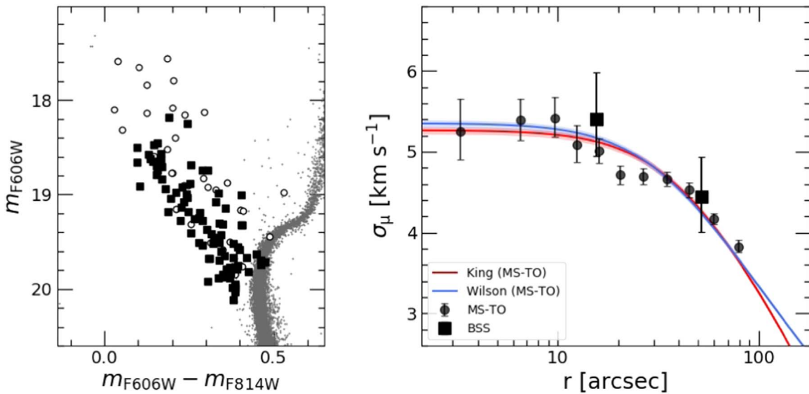
Figure 12. Left panel: CMD of NGC 1261, zoomed in around the BSS region. We show as black squares the BSSs used for the kinematic analysis and as empty circles those excluded because of too large PM errors. Right panel: BSS velocity dispersion profile (black squares). For comparison, we report the velocity dispersion profile of MS-TO stars and its best-fit King and Wilson models (red and blue lines, respectively), already shown in Figure 5.
