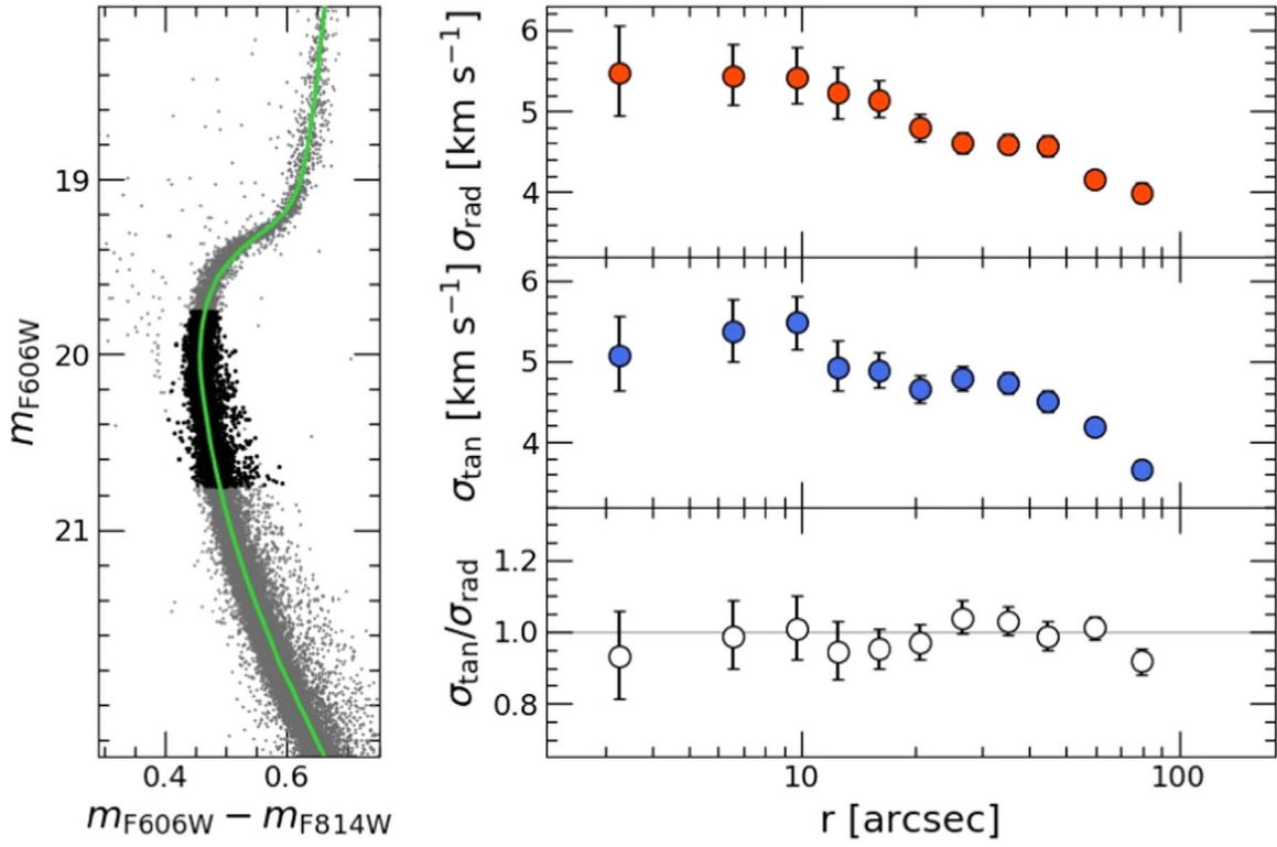
Figure 4. Left panel: CMD of NGC 1261 ( m_{F606W} vs. m_{F606W} - m_{F814W} ), using the quality-selected PM catalog (gray dots). The black points show the subsample of MS-TO stars selected to compute the velocity dispersion profiles. The green line is a PARSEC isochrone (Marigo et al. 2017), with an age of 11.5 Gyr and [\text{Fe}/\text{H}] = -1.35 (age and metallicity taken from Dotter et al. 2010). Right panels, from top to bottom: radial and tangential velocity dispersion profiles, and anisotropy profile (plotted, respectively, as red, blue, and white circles).
