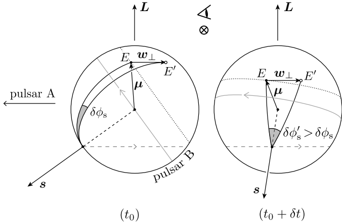
Fig. 10. Cartoon representation of spin-phase delay ( \delta\phi_s ) produced by the impact of the wind of pulsar A, with a perpendicular component to the LOS ( \mathbf{w}_\perp ) for two different phases of geodetic precession: at time ( t_0 ) and at a later time ( t_0 + \delta t ). In this representation, the observer's LOS is perpendicular to the plane of the figure, when looking down onto it; the plane of the orbit is perpendicular to the orbital angular momentum vector, \mathbf{L} ; and pulsar A is located to the left of pulsar B. The precession of the spin axis, \mathbf{s} , about \mathbf{L} , proceeds along the path shown with a dashed, grey line, in the direction indicated by the arrow. The NS's equator is shown with a solid, grey line, with the grey arrow indicating the spin direction; the magnetic axis, \boldsymbol{\mu} , rotates about the spin axis in the same direction. In both instances of time, the action of \mathbf{w}_\perp causes the deflection of the emission (assumed here to be at the magnetic pole) from position E (solid black point) to E' (open circle). The equivalent spin-phase delay, \delta\phi_s at ( t_0 ) and \delta\phi'_s at ( t_0 + \delta t ), is measured as the polar angle between E and E' . For the same wind magnitude ( w_\perp ), it can be seen that \delta\phi'_s > \delta\phi_s .
