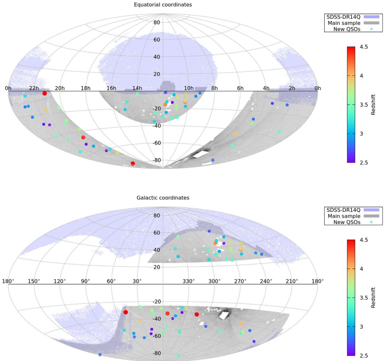
Figure 1. Maps of the locations of the sources in the main sample (Section 3.1, gray regions, a darker color indicates a higher density of sources). The locations of the QSOs in the SDSS DR14Q (P  ris et al. 2018) are represented by blue shaded regions. The new QSOs identified in this work are shown with filled circles, whose colors indicates the redshift. Upper panel: equatorial coordinates; lower panel: galactic coordinates.
