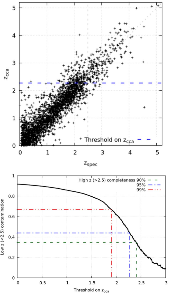
Figure 5. Upper panel: the z_{\text{cca}}-z_{\text{spec}} correlation (scatter: \sim 0.36 ). Lower panel: low- z ( < 2.5 ) “contamination” as a function of the adopted z_{\text{cca}} threshold and of the high- z ( > 2.5 ) “completeness” (dashed, dotted–dashed, and dotted–dotted–dashed lines). We chose a z_{\text{cca}} threshold of 2.27 corresponding to a high- z completeness of 95% and an expected low- z contamination in our final sample of \sim 44\% .
