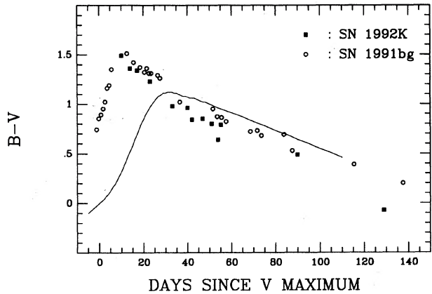
FIG. 6. The B-V color evolution of SNe 1992K and 1991bg along with the average color template curve calculated by Leibundgut (1988). The data for SN 1992K have been corrected for an assumed Galactic reddening of E(B-V)=0.12 .
