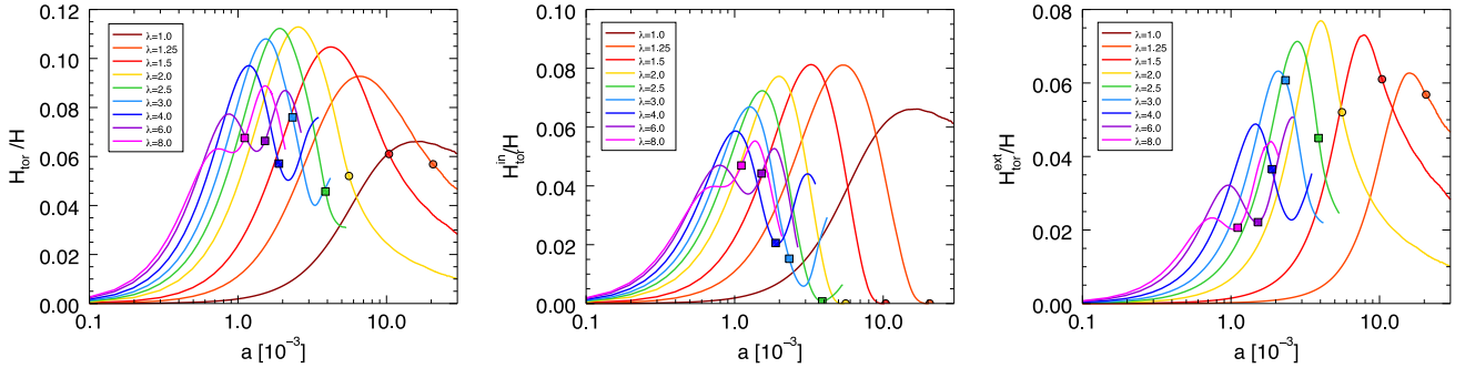
Figure 8. Profiles of the ratio of total magnetic energy of the toroidal component \mathcal{H}_{\text{tor}} , external one \mathcal{H}_{\text{tor}}^{\text{ext}} and internal one \mathcal{H}_{\text{tor}}^{\text{in}} , with respect to the total magnetic energy \mathcal{H} . The curves show sequences as a function of \hat{a} for various values of \lambda . The dots and squares as in Fig. 7.
