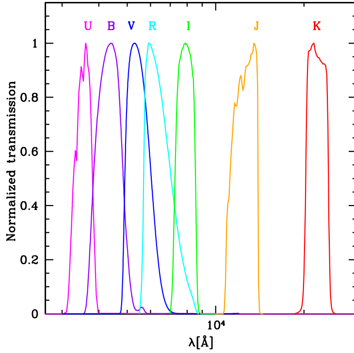
Figure 12. Filter curves over which rest-frame magnitudes have been computed following Methods 6a_{\tau} , 6a_{\tau}^{\text{NEB}} , 6a_{\text{del}\tau} and 6a_{\text{inv}\tau} . Filter curves are available as ascii files in the electronic version of the Journal.
