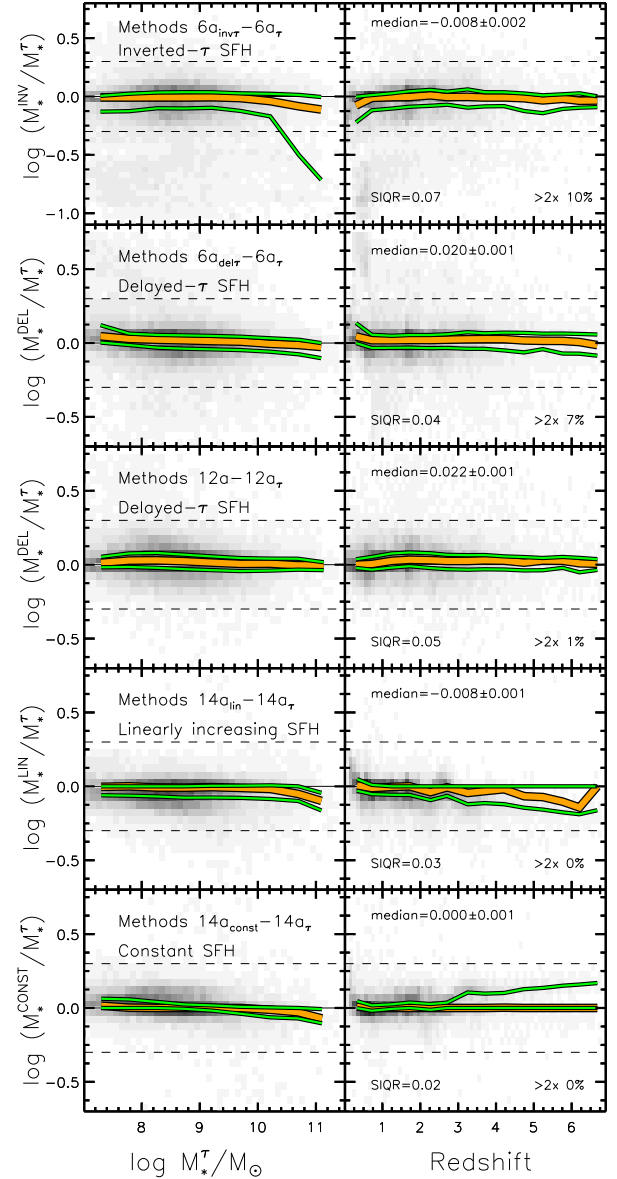
Figure 2. Comparison among stellar masses computed with consistent methods except for the choice of the SFH for the GOODS-S field. The ratio between masses computed with direct- \tau models ( M_*^\tau ), inverted- \tau models ( M_*^{\text{INV}} ), delayed- \tau models ( M_*^{\text{DEL}} ), linearly increasing models ( M_*^{\text{LIN}} ) and constant models ( M_*^{\text{CONST}} ) is studied against stellar mass ( M_*^\tau , left panels) and redshift (right panels). Colors show density of sources as in Figure 1. The thick orange lines show the median in bins of mass ( \Delta \log M_* = 0.5 ) or redshift ( \Delta z = 0.5 ), while the two thin green lines enclose 50% of the sample (representing the 25 ^{\text{th}} and 75 ^{\text{th}} percentiles in the same bins). The median logarithmic ratio with the associated error and the semi interquartile range (SIQR, see text) are printed in each panel, as well as the fraction of sources differing from the median value by more than a factor of 2 (i.e., falling beyond the dashed lines). The black solid line shows the locus where the two stellar masses are comparable. Delayed- \tau models in Method 6a _{\text{del}\tau} have a slightly different analytic shape ( \psi(t) \propto t^2/\tau \cdot \exp(-t/\tau) ) compared to Method 12a ( \psi(t) \propto t/\tau^2 \cdot \exp(-t/\tau) ).
