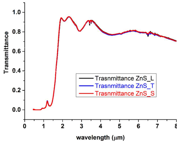
Figure 3: ZnS transmittance recorded using a parallel beam. The blue curve refers to the “T” sample, the red and black to the “S” and “L” respectively.
