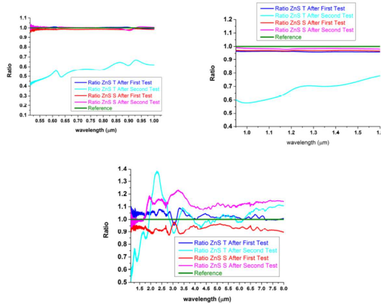
Figure 33: Ratio calculated for the reflectance according to the equation 2. The green curve is a reference while the blue and red curves are the ratio calculated after the first radiation test for the ZnS T and ZnS S respectively.
