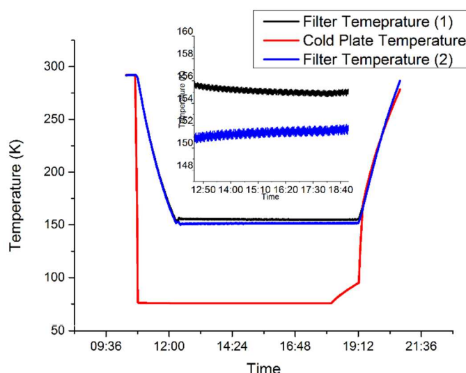
Figure 18 : Temperatures recorded during the irradiation test performed @ AOT. The red curve refers to the cold plate temperature, the blue and the black curves to the holder filter
