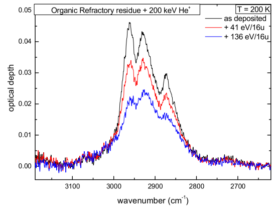
Fig. 7. Evolution of C-H stretching mode feature for the organic refractory residue: the initial stage is represented in black, and two steps of irradiation in red and blue. (For interpretation of the references to color in this figure legend, the reader is referred to the web version of this article.)
