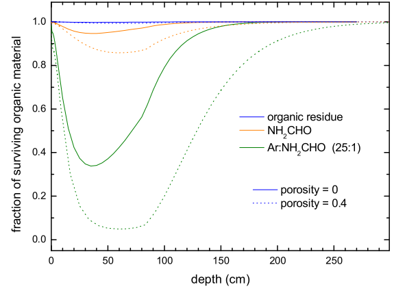
Fig. 11. Estimated fraction of surviving organic matter on the Moon as a function of depth. Three different values of destruction cross section and two different values of lunar regolith porosity were used.
