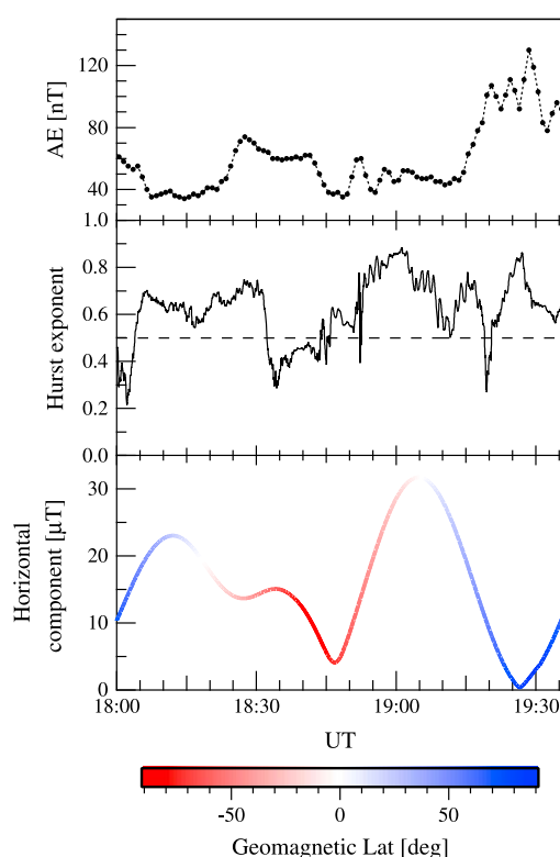
Figure 2. (top) The Auroral Electrojet (AE) index, (middle) the local Hurst exponent ( H ), and (bottom) the magnetic field horizontal component for an orbit of the Swarm A satellite on 1 April 2014. Dashed horizontal line (intermediate panel) is for H=0.5 and the color scale reported in the bottom plot shows the geomagnetic latitude of Swarm A during the selected orbit.
