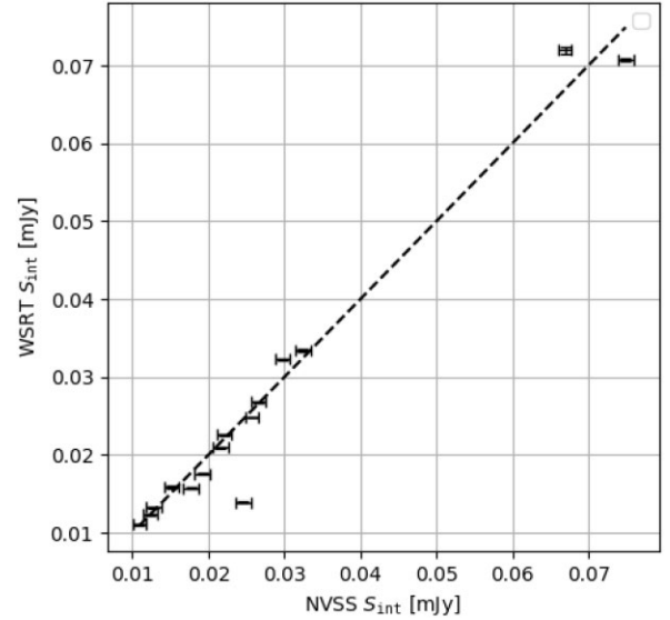
Figure 3. Cross-matched fluxes between WSRT 21 cm and the NVSS, integrated to the lower resolution of the NVSS. Error bars indicate 1\sigma fit errors taken from the PYBDSF catalogue fitting routine. Only sources above 20\sigma are shown. The WSRT 21 cm population was scaled to the NVSS frequency assuming a population spectral index of -0.7 , typical to AGN at this frequency.
