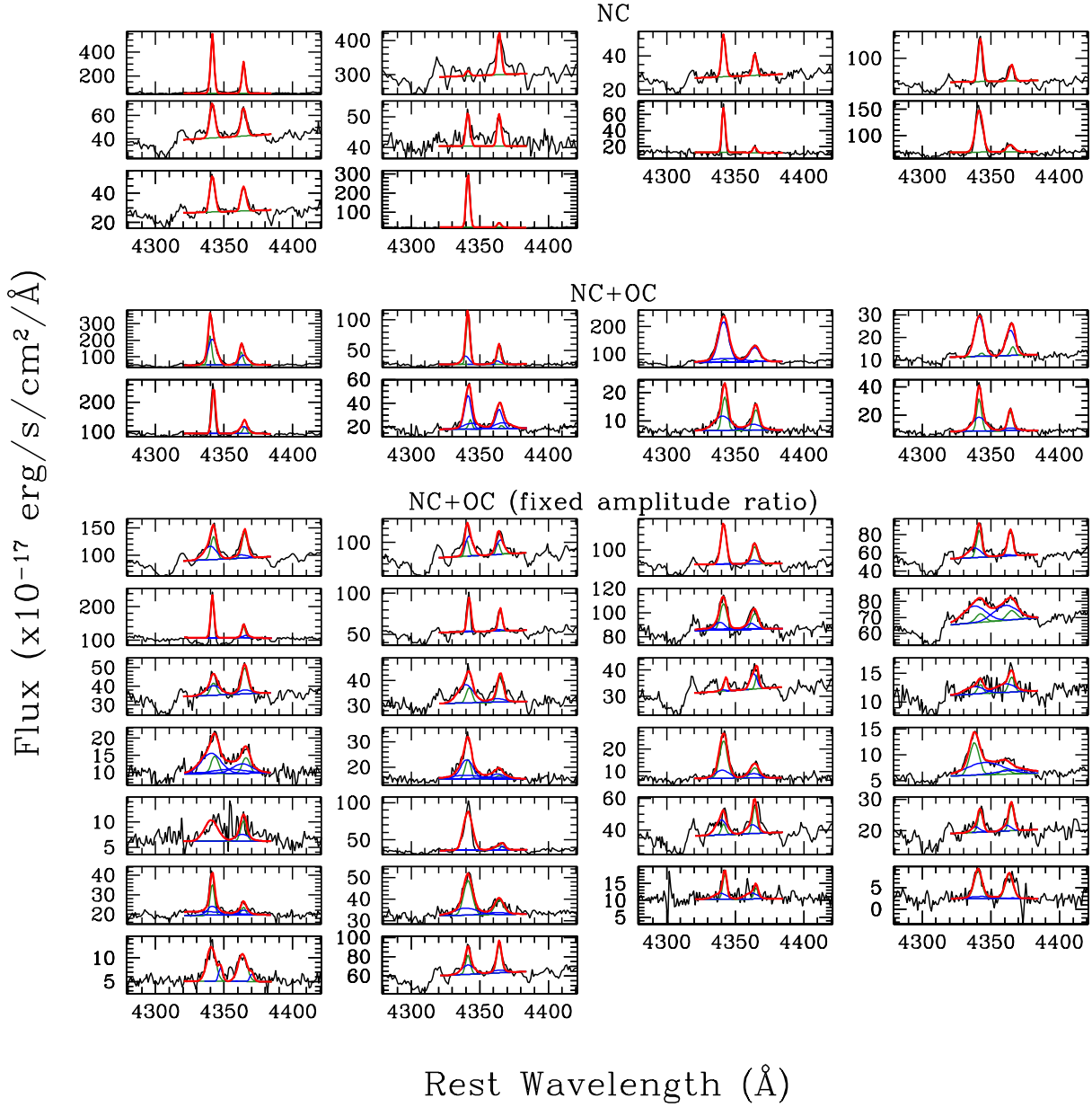
Fig. 3. Magnification of the region of [O III] \lambda 4363-H \gamma - \lambda 4342 lines for the 44 sources for which we could determine R_{[\text{OIII}]} flux ratios. For each spectrum, the best-fitting components presented in Sect. 3.1 are superimposed: solid green curves represent the systemic narrow component (NC); blue curves the OC.
