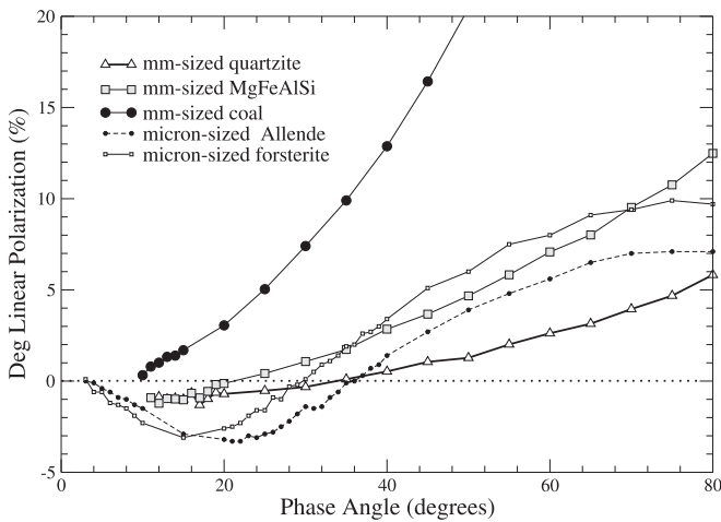
Figure 16. Measured negative polarization branches (in percentage), for the millimeter-sized compact particles and two micron-sized samples.
