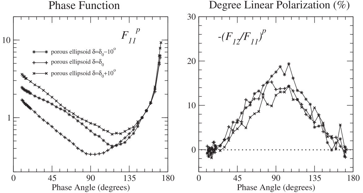
Figure 13. Measured phase function, F_{11}^p , and DLP (in percentage) curves, -(F_{12}/F_{11})^p , for a dirty highly porous ellipsoidal particle at three different orientations, p . The measured curves are presented with their error bars. In cases in which no error bars are shown, they are smaller than the symbol. The F_{11} curves are normalized to unity at 150^\circ .
