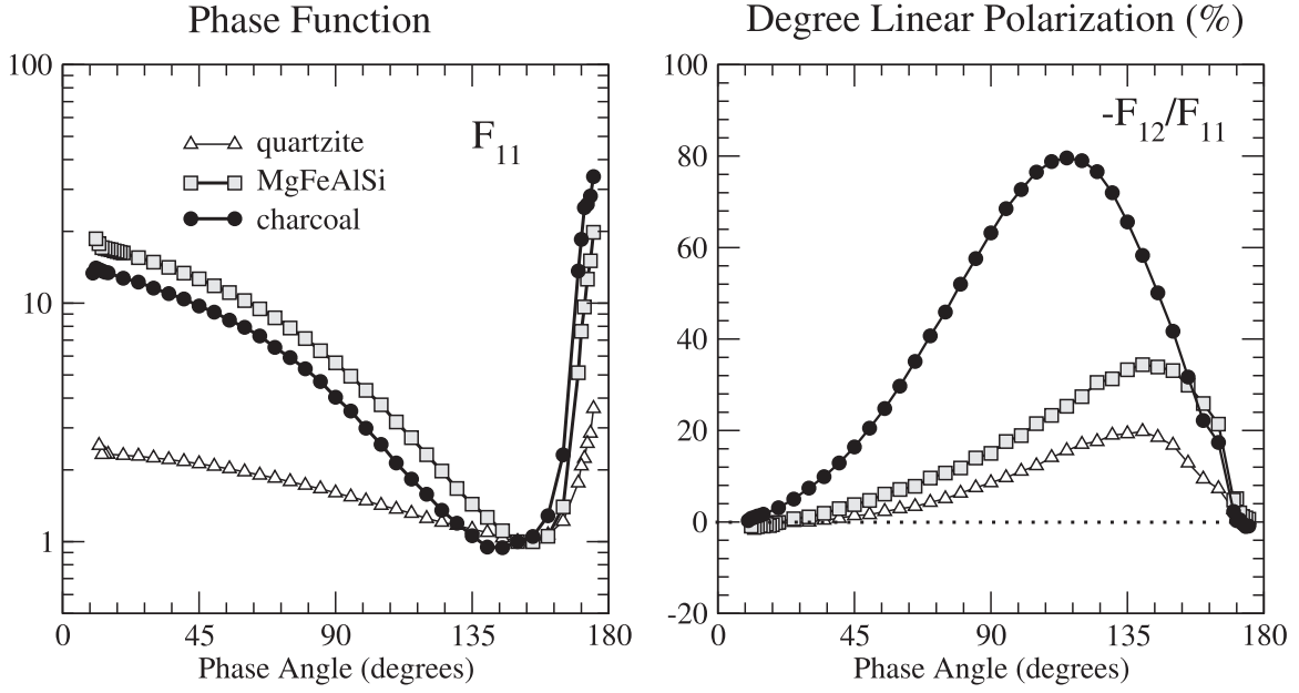
Figure 10. Experimental phase functions ( F_{11}(\theta) ) and DLP ( -F_{12}(\theta)/F_{11}(\theta) ) curves at 520 nm for charcoal (filled circles), MgFeAlSi (filled squares), and quartzite (triangles). All F_{11} curves are normalized to unity at 150°.
