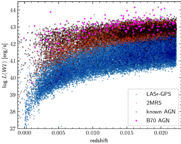
Figure 6. Central WISE WI luminosity over redshift for all galaxies from the 2MRS (orange) and LASr-GPS (blue). The semitransparent black crosses mark known AGN, while magenta crosses mark B70 AGN.
