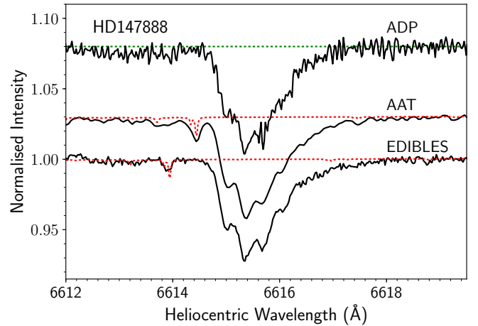
Fig. 12. Comparison of the 6614 Å DIB for HD 147888 ( \rho Oph D) obtained with EDIBLES (this work, R \sim 110\,000 ) and the AAT (Cordiner et al. 2013, R \sim 58\,000 ). The top spectrum labeled “ADP” is the spectrum obtained with the standard ESO archive pipeline processing (i.e. using the default number of 5 flat-field frames). The red dotted line represents the telluric absorption spectrum, shifted to match the heliocentric rest frame of each target; highlighting the presence of a small telluric absorption feature at 6614/6614.5 Å.
