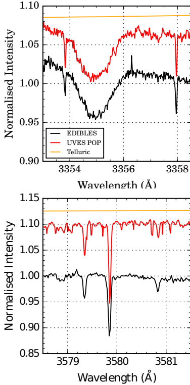
Fig. 13. Comparison of EDIBLES (black) and UVES POP (red) spectra of HD 169454 for interstellar lines of NH( \lambda\lambda 3353.92 , 3358.05 Å; top ) and CN( 1 - 0 ) ( \lambda\lambda 3579.45 , 3579.96 , and 3580.9 Å; Meyer et al. 1989; bottom ); the telluric spectrum is shown in orange. HD 169454 is a blue supergiant (B1 Ia) – the broad stellar line in the spectrum is He I \lambda 3355 Å.
