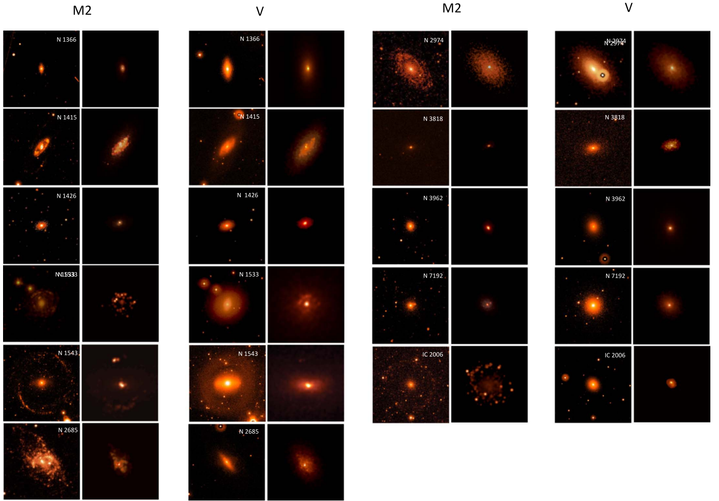
Figure 2. Observed vs. simulated image of the 11 galaxies. In each panel, the left column shows the Swift -UVOT M2- (first and fifth columns) or V- (third and seventh columns) band image; the right column shows the simulated image with the same field of view and resolution ( 1'' \text{ pixel}^{-1} ) of the observed one. All images are 5' \times 5' , except for NGC 1415 with 8.6' \times 8.6' and IC 2006 and NGC 2685 with 7' \times 7' .
