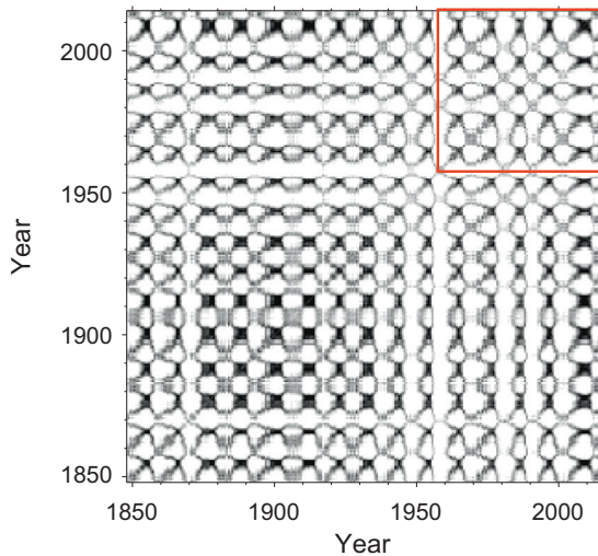
Fig. 3. RP of of the weekly unfiltered SSN1 (no embedding).
