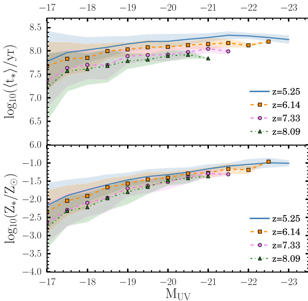
Figure 3. Mass-averaged stellar age (top panel) and metallicity (bottom panel) of the simulated galaxies as a function of their intrinsic UV magnitude ( \lambda = 1500 \text{ \AA} ). The different lines indicate the mean values at redshift \sim 5 (blue solid), 6 (orange dashed with squares), 7 (magenta dashed with dots) and 8 (green dotted with triangles). The shaded regions indicate the 1\sigma deviation. A coloured version of the figure is available online.
