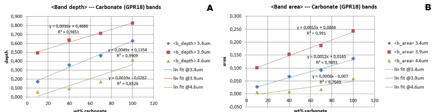
Fig. 15. Average band depth (A) and area (B) of carbonate absorption features centered at 3.4, 3.9 and 4.6 \mu\text{m} , vs. carbonate wt% content (GPR18) in the mixture set.
