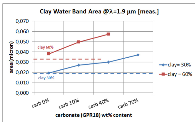
Fig. 14. Band area of 1.9 \mu\text{m} water absorption feature, due to clay. The addition of carbonate in the brucite–clay mixture causes the 1.9 \mu\text{m} band area to increase linearly with the carbonate content.
