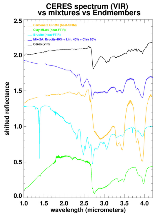
Fig. 17. Comparison between average spectrum of Ceres (Dawn-VIR, from De Sanctis et al., 2015) and endmembers. The spectrum has also been compared with a selected mixture, MIX-2A. The endmembers clay-MLA4 and brucite have been heated for 2.5 h at 250 ^{\circ}\text{C} , and then measured with FTIR, in order to reduce adsorbed water. The carbonate-GPR18 has been heated for 4.5 h at 150 ^{\circ}\text{C} and then measured with SPIM.
