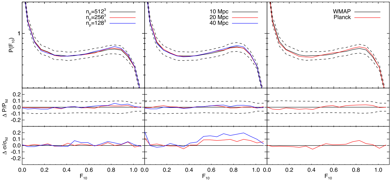
Figure C2. Convergence test of the transformed and regulated PDF in our hydrodynamical simulations. We show the effect of resolution (left), box size (middle) and cosmology (right). The upper panels show the PDFs of the fiducial runs and of the test runs, in the middle panels we plot the relative deviation of the PDF from the fiducial simulation, compared to the square root of the diagonal element of the covariance matrix (dashed black lines). In the bottom panel, we present instead the relative deviation of the diagonal errors. All the simulations used in this test have the smoothing parameter set to \xi = 1.45 . Left-hand panels: results for three simulations with box size 10 \text{ Mpc } h^{-1} with 512^3 (fiducial, black), 256^3 (red) 128^3 (blue) gas particles are shown. The PDF and the diagonal errors are converged to a few-per cent level. Central panels: The fiducial model is a 10 \text{ Mpc } h^{-1} simulation with 128^3 gas particles. We compare its PDF and the diagonal errors to those calculated from a 20 \text{ Mpc } h^{-1} simulation with 256^3 gas particles (in red), and a 40 \text{ Mpc } h^{-1} simulation with 512^3 particles (in blue). While the mean PDF is converged to a small fraction of the estimated uncertainty, the error themselves show a significant variation when the box size is increased. We correct the covariance matrix in our analysis to take this into account (see text). Right-hand panels: The black model uses the same cosmological parameter we have used throughout this paper, while the red curves are calculated assuming the best-fitting values from the first data release of Planck (Planck Collaboration XXXI 2014). The differences are always significantly smaller than the statistical errors.
