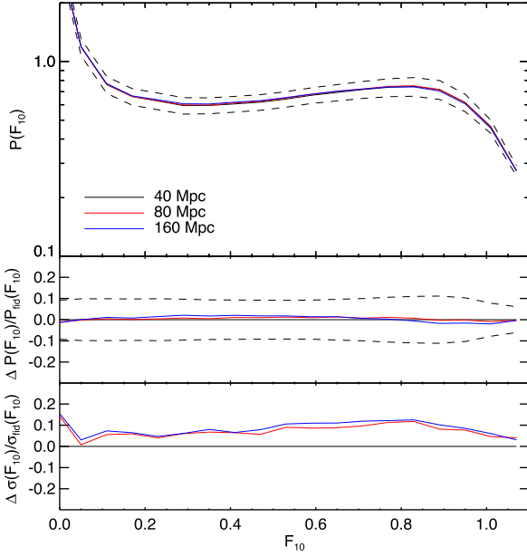
Figure D1. Same as the central panel of Fig. C2, but considering three runs from the Sherwood set of simulations (Bolton et al. 2016). The boxes are 40, 80 and 160 Mpc h^{-1} of size with 2 \times 512^3 , 1024^3 , 2048^3 particles, respectively, which matches the resolutions of the simulation shown in Fig. C2. Compared to the previous test on smaller boxes, the convergence of the errors is significantly improved, down to a level of 5 per cent at most for the 80 Mpc h^{-1} box (we remind the reader that the F_{10} = 0 bin is excluded from the analyses). We reckon that this level of convergence is satisfactory for the degree of precision of this work, and a slight change in our covariance estimate would not qualitatively modify any of our conclusions.
