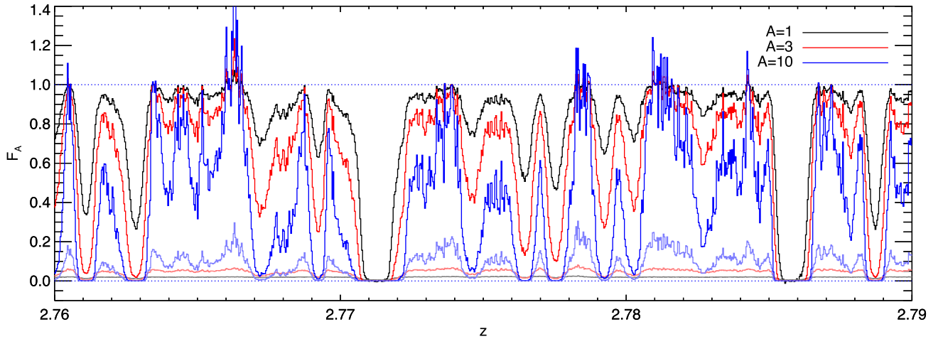
Figure 4. The effect of rescaling the optical depth for a selected chunk of the Ly \alpha forest of the DEEP spectrum. The plot shows the transformed flux F_A after multiplying \tau by a factor A = 1 (black, original spectrum), 3 (red) and 10 (blue). The spectrum is continuum-regulated before applying the transformation, so that 5 per cent of the pixels have flux above 1, explaining the occasional spikes in the transformed flux. The propagated instrumental errors after the transformation are shown as lighter lines at the bottom, matched by colour to the transformed fluxes. The motivation for applying this transformation is that it amplifies fluctuations near the continuum as A increases, while the most absorbed regions, corresponding to high densities, become saturated. This mimics what happens in a denser universe or with a lower amplitude UV background, resembling the Ly \alpha forest at higher z . In this way, we are able to increase our sensitivity to the low-density regions of the IGM, which are difficult to probe otherwise.
