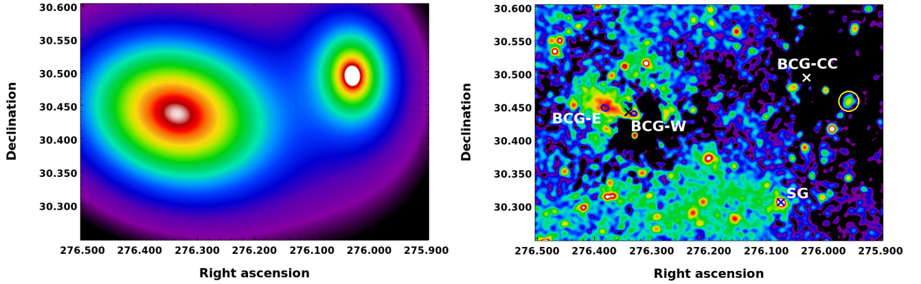
Fig. 3. Left panel: surface brightness model that includes both elliptical single \beta -models of RXCJ1825 and CIZA1824 clusters. Right panel: residual image after subtracting the model from the X-ray image. Blue small ellipses show the position of the two BCGs of RXCJ1825, labeled BCG-W and BCG-E, and the black cross is the X-ray centroid of the cluster. The white and blue crosses show the position of the BCG of CIZA1825, BCG-CC, and of the SG, respectively.
