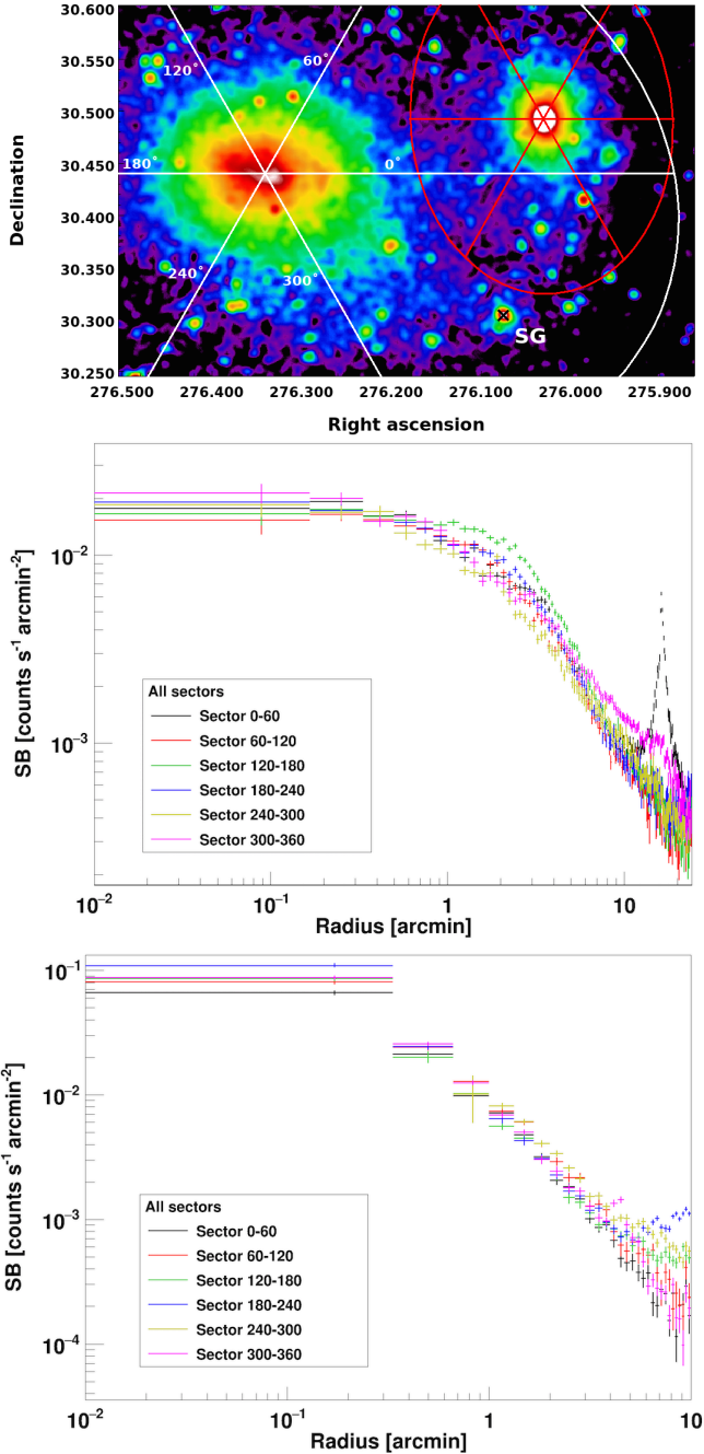
Fig. 2. Top panel: elliptical sectors (60° wide) used for the extraction of surface brightness profiles, overplotted on the XMM-Newton mosaic image (Fig. 1). The orientation angle is calculated counterclockwise from the Right Ascension axis. Middle and bottom panels: elliptical surface brightness profiles of RXCJ1825 and CIZAJ1824 extracted in the sectors, respectively. In the x-axis we plot the distances along the major axis of the ellipses. Point-like sources are removed. The black cross shows the position of the SG. The features seen in the profiles are described in Sect. 3.1.1.
