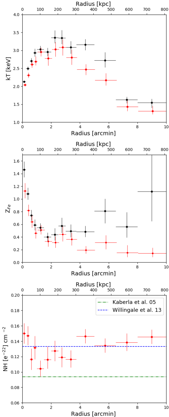
Fig. 10. Radial temperature ( upper panel ) and metal abundance ( middle panel ) profiles of CIZA J1824. Black points show the results from the standard analysis with NH fixed to the LAB value and energy band [0.5–10] keV and red points show the results with NH left free to vary in the fit (the points of each bin have been shifted slightly for visual clarity). Lower panel : galactic hydrogen column density profile of CIZA J1824. The green dot-dashed line is the NH LAB value (Kaberla et al. 2005), and the blue dashed line is the total NH (NHI + NHII) value taken from Willingale et al. (2013).
