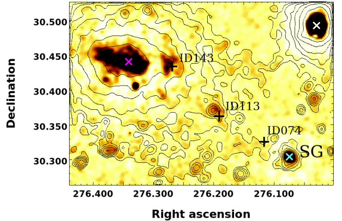
Fig. 18. Unsharp-mask image of the Lyra complex with the high-velocity galaxies selected by Girardi et al. (2019) shown as black crosses (ID143, ID113, and ID074 in Table 6 of Girardi et al. 2019). The magenta, white, and cyan crosses are the X-ray centroid of RXCJ1825, the BCG-CC, and the SG, respectively. Black contours are the surface brightness levels.
