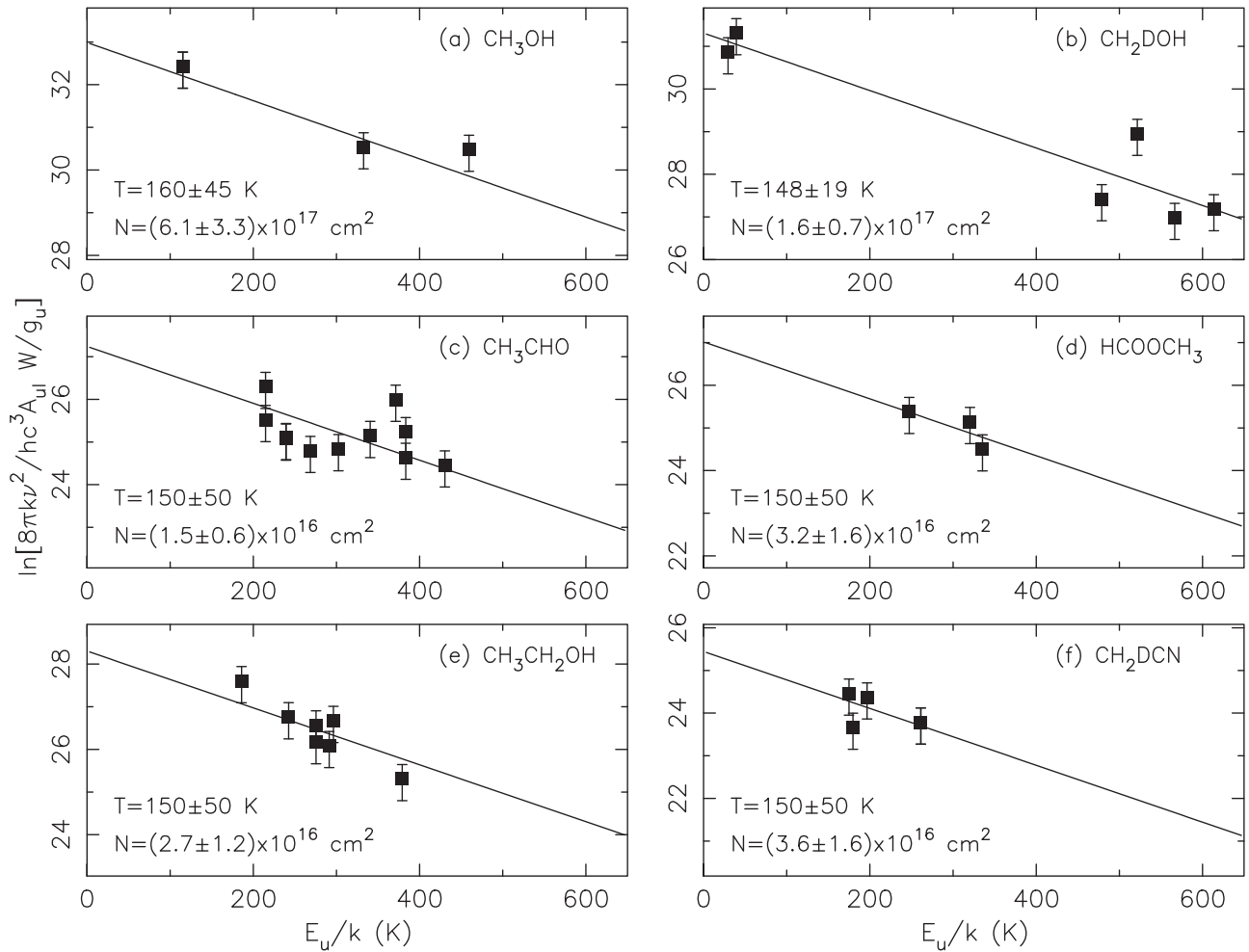
Figure 3. Rotation diagrams for molecular lines of the six organic molecules including \text{CH}_3\text{OH} , \text{CH}_2\text{DOH} , \text{CH}_3\text{CHO} , \text{HCOOCH}_3 , \text{CH}_3\text{CH}_2\text{OH} , and \text{CH}_2\text{DCN} . The diagrams are derived from the line intensities in the lower disk atmosphere listed in Table 1. The error bars show the uncertainty in our measurements, which are assumed to be 40% of the data values. The solid line is a linear fit to the data. In panels (c)–(f), the temperature is fixed at 150 \pm 50 K for the fitting in order to derive the column densities from the weak lines.
