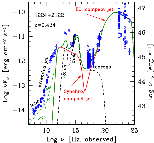
Figure 1. SED of CRATES J1224+2122 (alias PKS 1222+21 alias 4C +21.35), a Fermi /Large Area Telescope (LAT) detected blazar (Shaw et al. 2012). The solid red line is the emission from the single-zone jet model we adopted (see text and Ghisellini & Tavecchio 2015), the short-dashed black line is the contribution from the thermal components (i.e. accretion disc, the torus and the X-ray corona), while the solid green line is the sum of the two. The adopted jet model assumes that most of the emission comes from a compact jet region, and therefore the synchrotron emission is self-absorbed up to \sim 10^3 GHz. At lower frequencies, the flux is produced by several larger jet regions, self-absorbing at smaller frequencies, and by the extended radio-lobes, whose synchrotron emission is optically thin. The latter component is relatively steep ( F_\nu \propto \nu^{-0.7} ), while the partially opaque emission from the jet is flat ( F_\nu \propto \nu^0 ), as illustrated by the long-dashed green lines.
