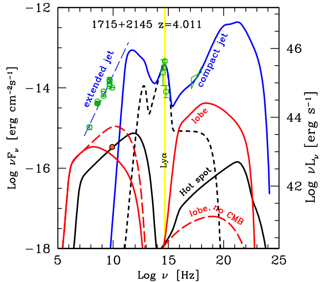
Figure 3. SED of 1715+2145, together with the models for the different components of the emission: (i) the thermal component, namely the accretion disc, the torus and the X-ray corona (short-dashed black line); (ii) the emission from the compact and relativistically beamed jet (the blue solid line is the sum of the jet and the thermal components), accounting for most of the emission, but not for the radio flux, that must be produced by more extended regions (but still relativistic) of the jet, forming the flat radio spectrum; (iii) the emission from the hotspots (solid black line) assumed to have a radius of R_{\text{spot}} = 1.5 \text{ kpc} , as measured by VLA (Gobeille et al. 2014); (iv) the lobe emission (solid red line), assuming that the power injected throughout the lobe in the form of relativistic electrons is P_{\text{e,lobe}} = 0.1 P_{\text{jet}} . Magnetic and electron lobe energies are in equipartition. For illustration, the dashed red line shows the lobe emission for the same P_{\text{e,lobe}} and magnetic field, but now neglecting the effects of CMB photons. The long-dashed blue line is not a fitting model, but simply a line to guide the eye. See Table 2 for the adopted parameters. Data points are from the ASDC archive, the bow tie in X-rays is from Wu et al. (2013). The orange circle corresponds to 4 mJy at 8.4 GHz, and is the flux observed by the two hotspots. The vertical yellow line flags the position of the \text{Ly}\alpha line. Above this line the flux is severely absorbed by the intervening matter, and we do not consider the corresponding data in the fit. (see for illustration the case of 1026+2542 in Fig. 8).
