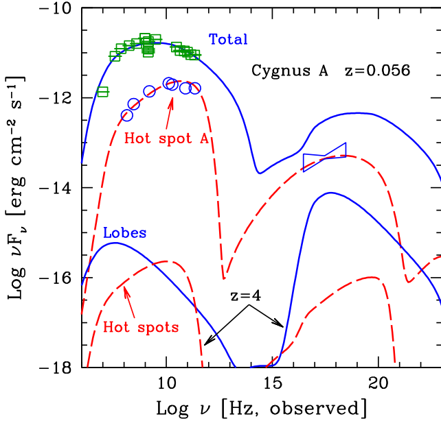
Figure 2. SED of the hotspot A (the brightest) of Cygnus A (blue circles), compared to the total radio emission (green squares). The blue bow tie refers to the X-ray flux of the hotspot A as observed by Chandra (Wilson et al. 2000). The dashed red and solid blue lines are the corresponding SSC models. For simplicity, we have fitted the total emission with the lobe model. The bottom lines show how the emission of the lobes and the hotspots would appear if the source were at z = 4 .
