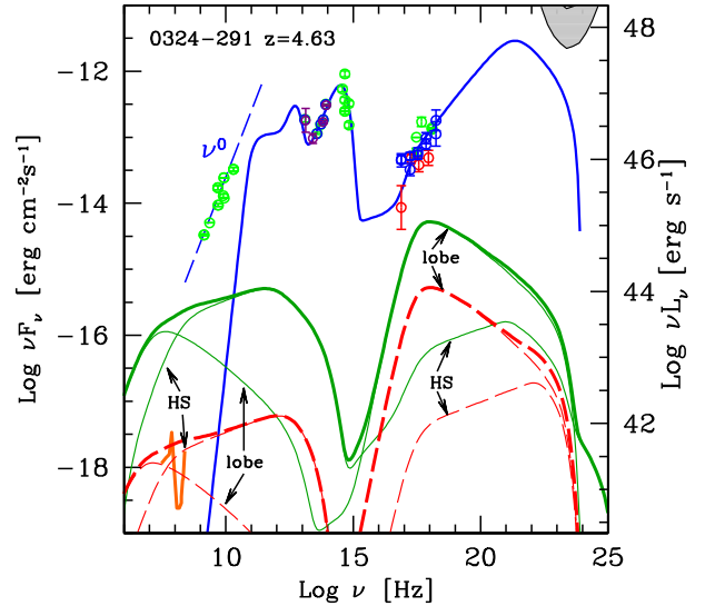
Figure 7. SED of the blazar 0324–291. The blue solid line is the model for the sum of jet emission and thermal components (see Fig. 1). For the hotspots and the lobes, we show two possible models: one with 0.1 P_{jet} (thin green lines) and the other with 0.01 P_{jet} (thin red lines). We show separately the contribution of the hotspots and the lobes, as labelled, while the thick green and red lines are the corresponding sums. The radius of the hotspots and the lobes are assumed to be R_{HS} = 2 kpc and R_{lobe} = 50 kpc. The straight dashed blue line interpolating the radio spectrum is not a fit, but only a guide to the eye. The hatched grey area in the upper right corner shows the sensitivity of Fermi /LAT ( 5\sigma ) after 5 yr of observing time. We also report (orange line) the sensitivity of LOFAR.
