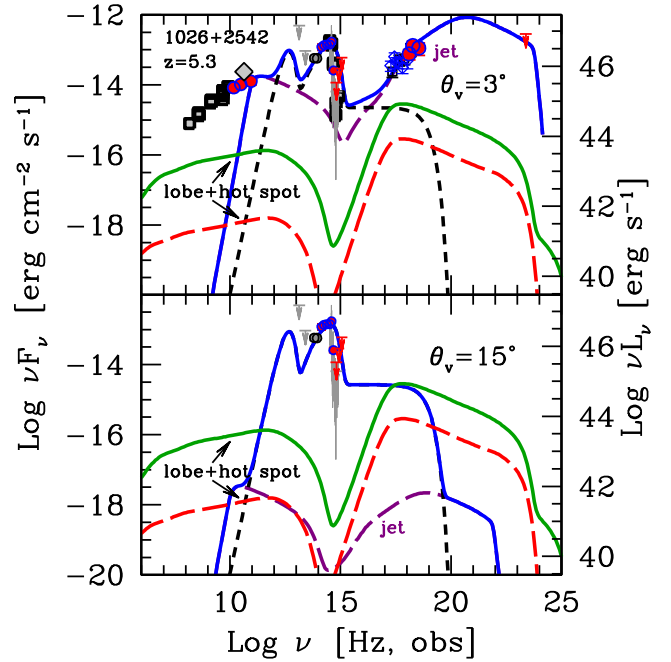
Figure 9. Top panel: the SED of the blazar 1026+2542 at z = 5.3 is fitted with a model (parameters in Table 3) with \Gamma = 15 and \theta_v = 3^\circ , as in Fig. 8. Here we also show the contribution from the jet (long-dashed violet line), the thermal components (disc, torus and corona, as a short-dashed black line) and their sum (solid blue line). The solid green and the dot-dashed red lines are the estimated lobe + hotspot emission as in Fig. 8 (the two models differ from the assumed injected electron energy, equal to 10 per cent of 1 per cent of P_{\text{jet}} , respectively). Bottom panel: if the very same source is observed at \theta_v = 15^\circ (i.e. only slightly off the beaming angle), the jet emission (long-dashed red line) is so weak that it would be missed by all current surveys, while the isotropic components (disc, torus, corona and the lobes) would remain the same. Current optical surveys, as the SDSS, would easily detect the source, and classify it as a radio-quiet quasar. The lobe + hotspot emission, slightly below the sensitivity of FIRST (1 mJy at 1.4 GHz), could be detectable by LOFAR (see Fig. 8); furthermore, pointed Chandra X-ray observations could detect and resolve the X-ray emission of the lobes (note that 50 kpc at z = 5.3 correspond to an angular size of 8.2 arcsec in the adopted cosmology). These observations could establish the jetted nature of the source.
