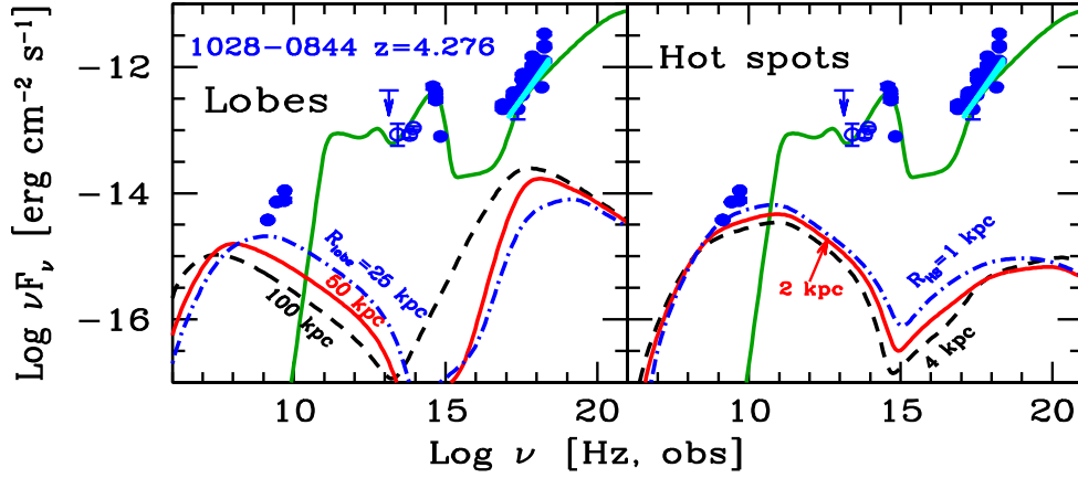
Figure 4. Predicted lobe and hotspot emission from the blazar 1028–0844. The left-hand panel shows the lobe emission for R_{\text{lobe}} = 100 kpc (short-dashed black line), R_{\text{lobe}} = 50 kpc (solid red) and R_{\text{lobe}} = 25 kpc (dot-dashed blue). For all cases, we have assumed that the jet deposits in relativistic electrons the same power, i.e. 0.1P_e^{\text{jet}} = 2.7 \times 10^{46} erg s ^{-1} for each lobe and hotspot. For the right-hand panel, the hotspot radius R_{\text{HS}} = 4 kpc (dashed black line), R_{\text{HS}} = 2 kpc (solid red) and R_{\text{HS}} = 1 kpc (dot-dashed blue). The magnetic field is found imposing equipartition with the total electron energy, both for the lobe and for the hotspot. The green solid line refers to the jet model (as in Figs 5 and 6). See Table 2 for the adopted parameters.
