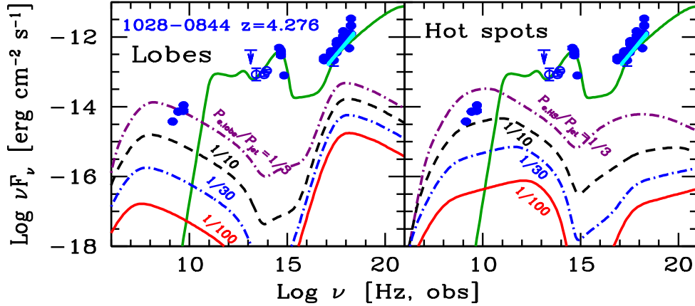
Figure 5. Predicted lobe and hotspot emission from the blazar 1028–0844 as a function of the injected power in relativistic electrons. For both panels P_e/P_{\text{jet}} = 1/3 (violet dot-dashed line); 1/10 (dashed black line); 1/30 (dot-dashed blue line) and 1/100 (solid red line). For all cases, we have assumed that the lobe radius is 50 kpc and the hotspot radius is 2 kpc. The magnetic field is found imposing equipartition with the total electron energy. A larger P_e implies a larger equipartition magnetic field and this in turn implies that the synchrotron luminosity increases more than the inverse Compton one. See Table 2 for the adopted parameters.
